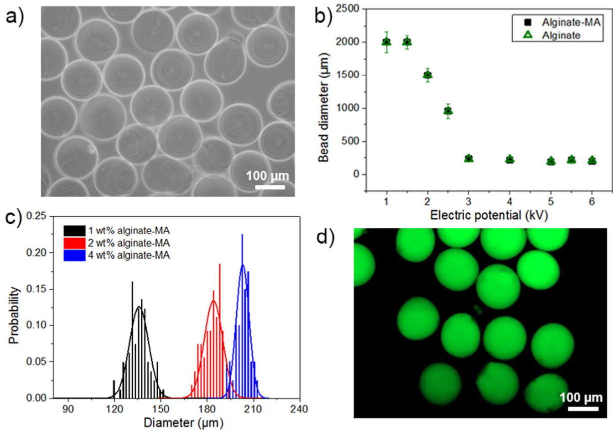
Figure 3. a) Optical microscopy image of 2 wt% alginate-MA beads at electric potential of 6.0 kV; b) Plot of bead diameters for 2 wt% alginate and alginate-MA for different applied electric potential, the data are presented as arithmetic mean \pm standard deviation calculated from at least three replicates; c) Bead diameter distribution of 1 wt%, 2 wt%, and 4 wt% alginate-MA at electric potential of 6.0 kV; d) Fluorescence microscopy image of 2 wt% fluorescein-labelled alginate-MA beads, beads were formed at electric potential of 6.0 kV.
