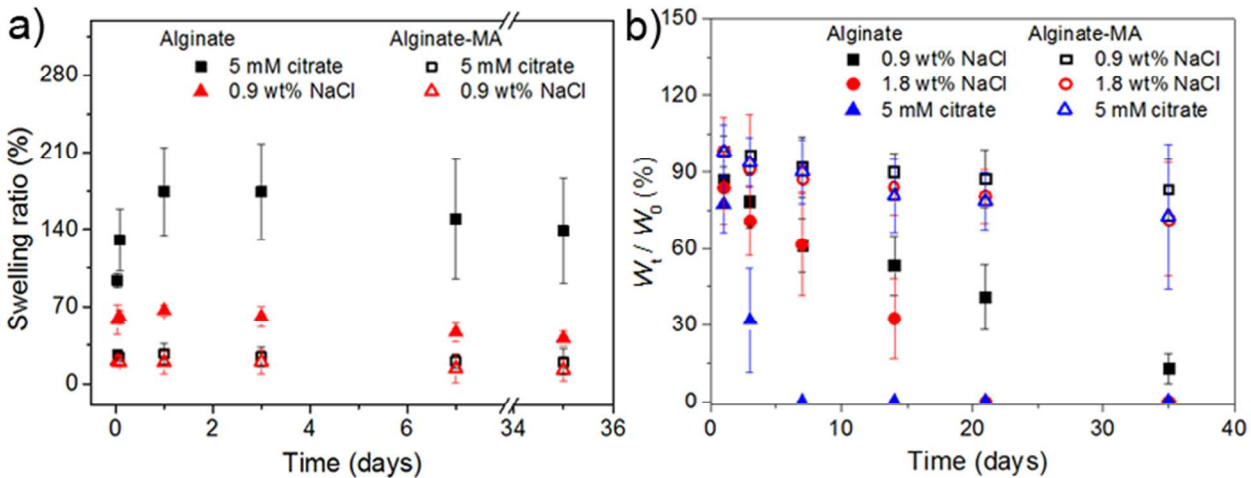
Figure 4. a) Swelling ratio of alginate and alginate-MA beads in 5 mM sodium citrate and 0.9 wt% NaCl solution vs. time. The data are presented as arithmetic mean \pm standard deviation calculated from at least 50 randomly chosen microbeads from microscopy images; b) Ratio between dried bead weight at time t and dried bead weight at time 0 in 0.9 wt%, 1.8 wt%, and 5 mM citrate solution. The solution was changed at every measured time point. The data are presented as arithmetic mean \pm standard deviation calculated from at least three technical replicates.
