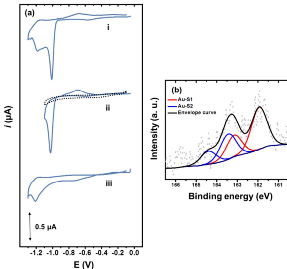
Figure 4. (a) Reductive desorption of MCH formed on Au electrodes (1 mm diameter) patterned with SU-8 photolithography: (i) full: in the potential range of 0 V – 1.3 V, (ii) partial: in the potential range of 0 V – -1.1 V (1 st cycle – solid line; 10 th cycle – dashed line) and (iii) desorption in the potential range of 0 V – 1.3 V after partial desorption in the potential range of 0 V – 1.1 V. The scan direction was negative, the scan rate was 100 mV/s and the scans were initiated at the potential of 0 V vs. Ag/AgCl/saturated KCl. (b) S2p spectrum of MCH on Au electrode surface after reductive desorption in the potential range of 0 V – 1.1 V.
