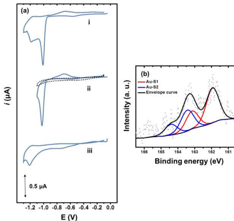
Figure 4. (a) Reductive desorption of MCH formed on Au electrodes (diameter 1 mm) patterned with SU-8 photolithography: (i) full: in the potential range of 0 V – 1.3 V, (ii) partial: in the potential range of 0 V – -1.1 V (1 st cycle – solid line; 10 th cycle – dashed line) and (iii) desorption in the potential range of 0 V – 1.3 V after partial desorption in the potential range of 0 V – 1.1 V. The scan direction was negative, the scan rate was 100 mV/s and the scans were initiated at the potential of 0 V vs. Ag/AgCl/saturated KCl. (b) S2p spectrum of MCH on Au electrode surface after reductive desorption in the potential range of 0 V – 1.1 V.
