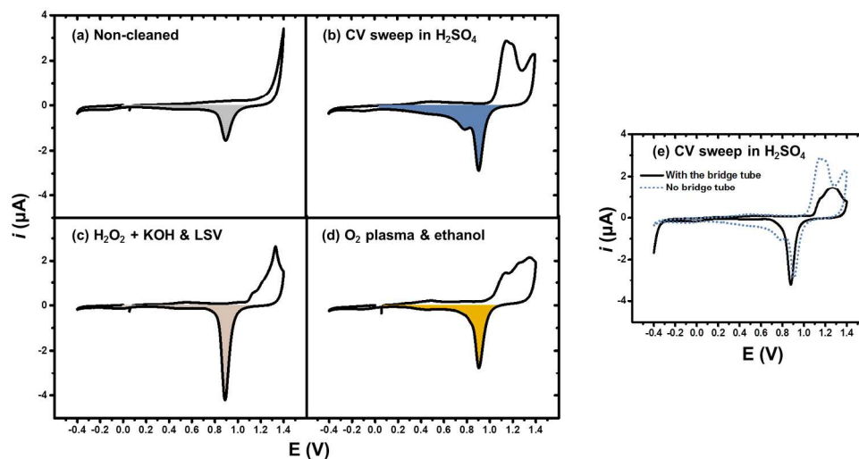
Figure 2. Cyclic voltammograms recorded in 50 mM \text{H}_2\text{SO}_4 for Au electrodes (1 mm diameter) patterned with SU-8 photolithography before and after using different pretreatment methods: (a) non-cleaned, (b) after "CV sweep in \text{H}_2\text{SO}_4 ", (c) after " \text{H}_2\text{O}_2 + KOH & LSV" and (d) after " \text{O}_2 plasma & ethanol", (e) after "CV sweep in \text{H}_2\text{SO}_4 " with and without the bridge tube. The integrated current profile areas are depicted in color. The scan direction was positive and the scans were initiated at the potential of 0 V vs. Ag/AgCl/saturated KCl.
