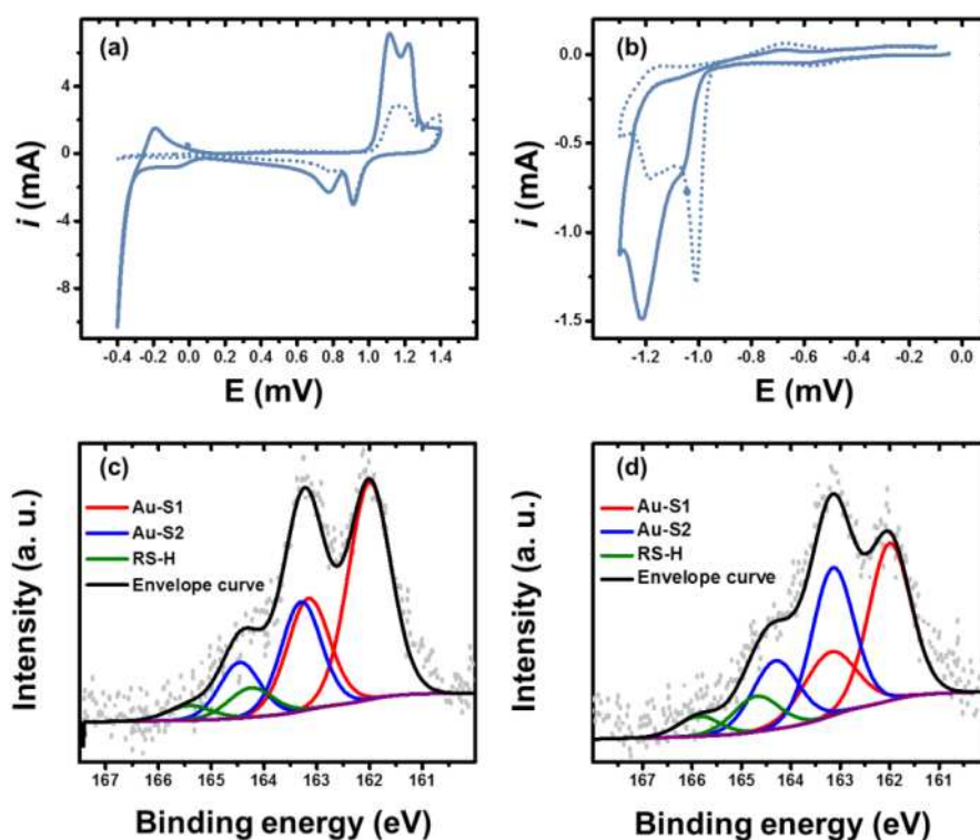
Figure 5. (a) Cyclic voltammograms recorded in 50 mM H 2 SO 4 using bare Au electrodes (diameter 1 mm) patterned with SU-8 photolithography and (b) reductive MCH desorption in 100 mM KOH after surface pretreatment by the “CV sweep in H 2 SO 4 ” for 15 (dotted line) and 50
