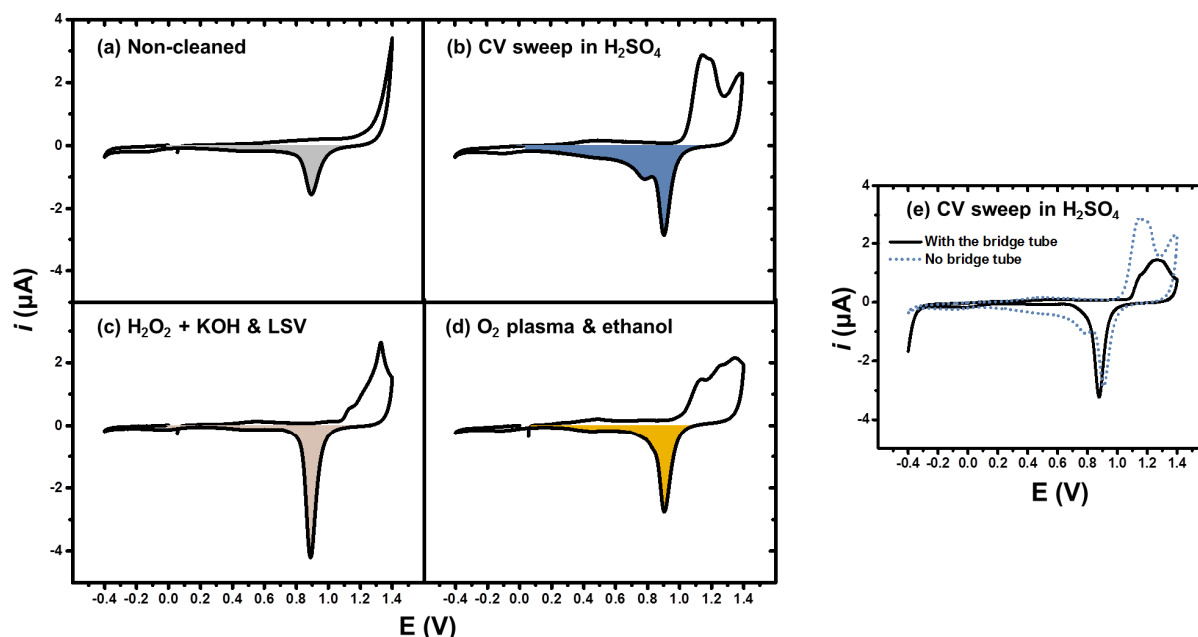
Figure 2. Cyclic voltammograms recorded in 50 mM \text{H}_2\text{SO}_4 for Au electrodes (diameter 1 mm) patterned with SU-8 photolithography before and after using different pretreatment methods: (a) non-cleaned, (b) after “CV sweep in \text{H}_2\text{SO}_4 ”, (c) after “ \text{H}_2\text{O}_2 + \text{KOH} + \text{LSV} ” and (d) after “ \text{O}_2 plasma & ethanol”, (e) after “CV sweep in \text{H}_2\text{SO}_4 ” with and without the bridge tube. The integrated current profile areas are depicted in color. The scan direction was positive and the scans were initiated at the potential of 0 V vs. Ag/AgCl/saturated KCl.
