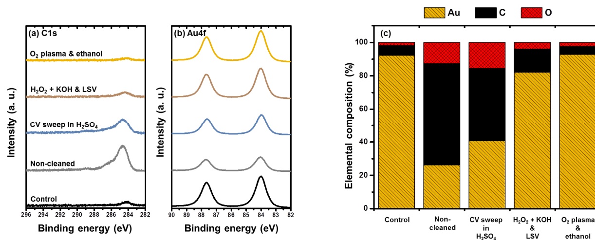
Figure 1. (a) C1s and (b) Au4f spectra and (c) elemental composition of Au electrode (diameter 1 mm) surfaces patterned with SU-8 photolithography before and after pretreatments of “KOH + H 2 O 2 & LSV”, “CV sweep in H 2 SO 4 ” and “O 2 plasma & ethanol”.
