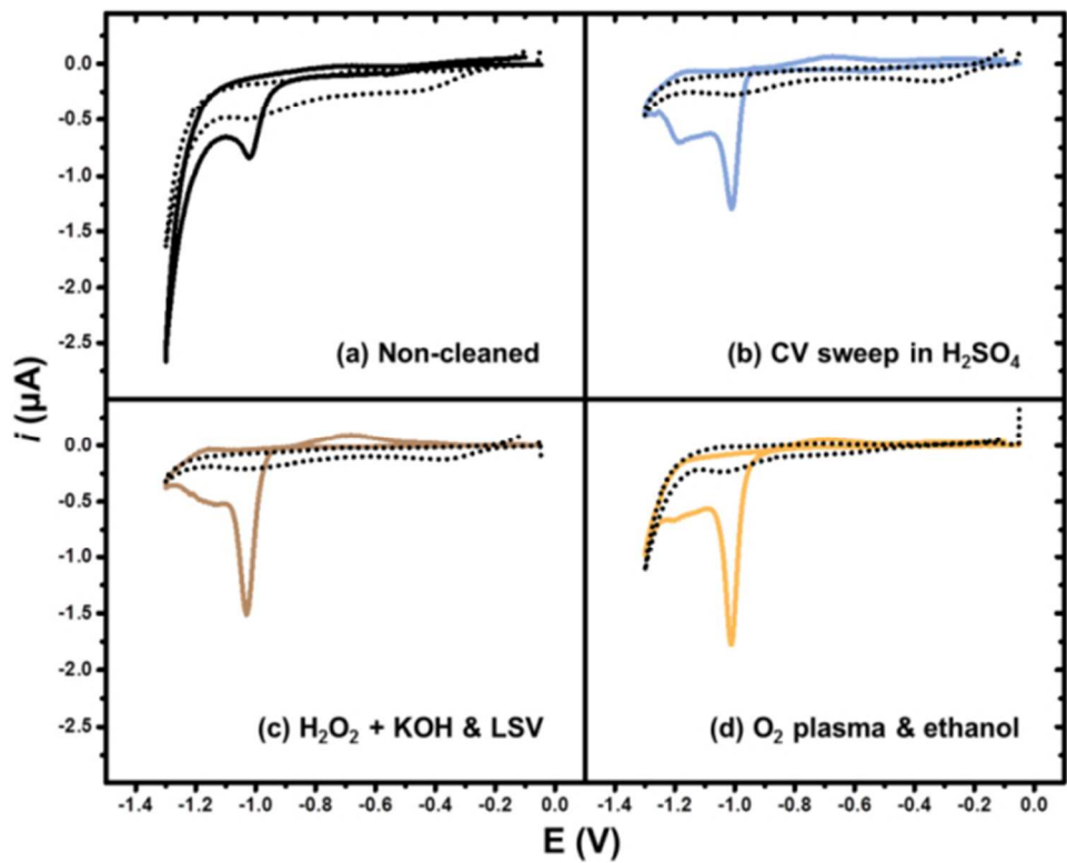
Figure 3. Reductive desorption of MCH (solid line) formed on Au electrodes (1 mm diameter) patterned with SU-8 photolithography after using different surface pretreatments: (a) non-cleaned, (b) after "CV sweep in H_2SO_4 ", (c) after " H_2O_2 + KOH & LSV" and (d) after " O_2 plasma & ethanol". The background current is depicted in a dotted line. The electrolyte was 100 mM KOH. The scan direction was negative, the scan rate was 100 mV/s and the scans were initiated at the potential of 0 V vs. Ag/AgCl/saturated KCl.
