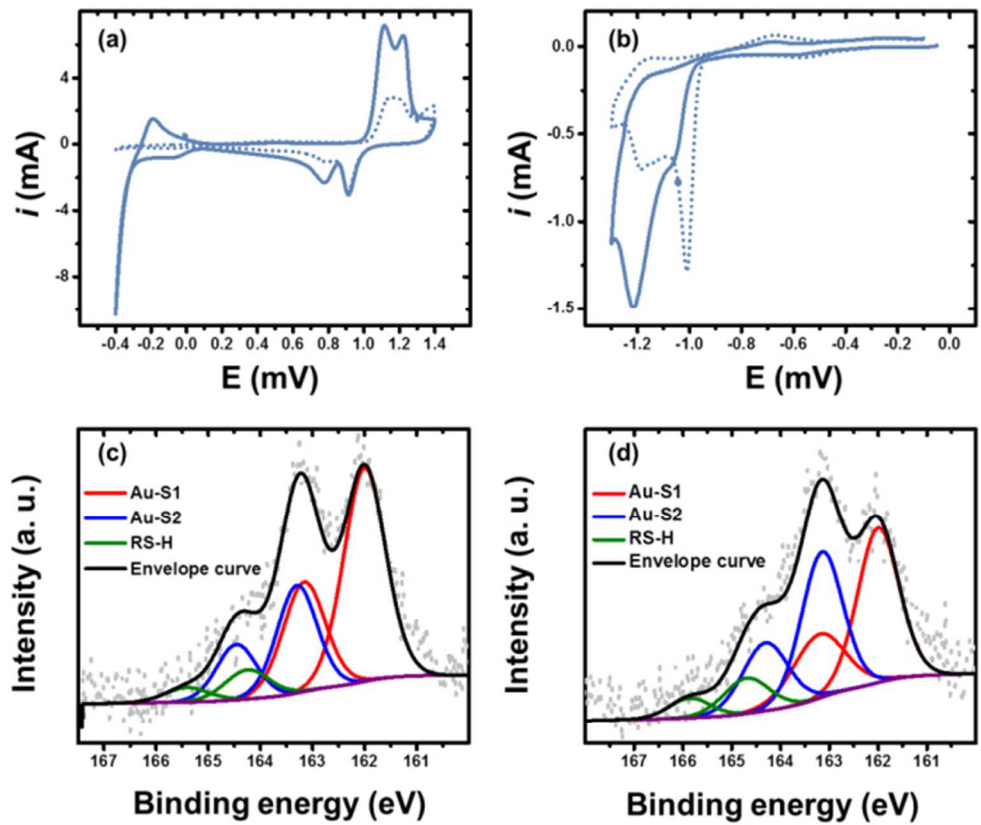
Figure 5. (a) Cyclic voltammograms recorded in 50 mM H_2SO_4 using bare Au electrodes (1 mm diameter) patterned with SU-8 photolithography and (b) reductive MCH desorption in 100 mM KOH after surface pretreatment by the “CV sweep in H_2SO_4 ” for 15 (dotted line) and 50 (solid line) cycles. The scan rate was 100 mV/s. XPS S_{2p} spectra of MCH adsorbed on Au electrodes pretreated by “CV sweep in H_2SO_4 ” for (c) 15 and (d) 50 cycles.
