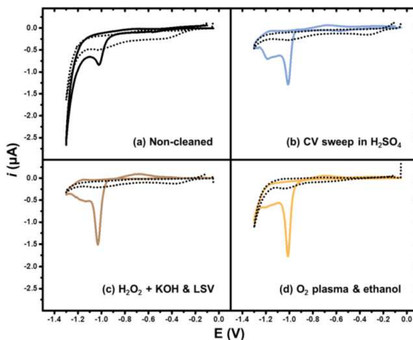
Figure 3. Reductive desorption of MCH (solid line) formed on Au electrodes (diameter 1 mm) patterned with SU-8 photolithography after using different surface pretreatments: (a) non-cleaned, (b) after “CV sweep in \text{H}_2\text{SO}_4 ”, (c) after “ \text{H}_2\text{O}_2 + \text{KOH} + \text{LSV} ” and (d) after “ \text{O}_2 plasma & ethanol”. The background current is depicted in a dotted line. The electrolyte was 100 mM KOH. The scan direction was negative, the scan rate was 100 mV/s and the scans were initiated at the potential of 0 V vs. Ag/AgCl/saturated KCl.
