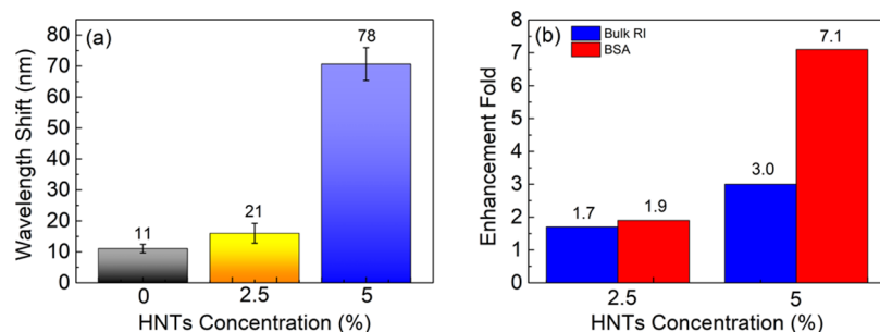
Figure 8. (a) Resonance wavelength shift for the control SPR sensor and HNTs-SPR sensors modified with different concentrations of HNTs, when flowed through phosphate buffer and BSA solutions ( \sim 1 mg/mL) successively. (b) Comparison of the sensitivity enhancement fold for the HNTs-SPR sensor when tested in bulk RI solutions and BSA solutions.
