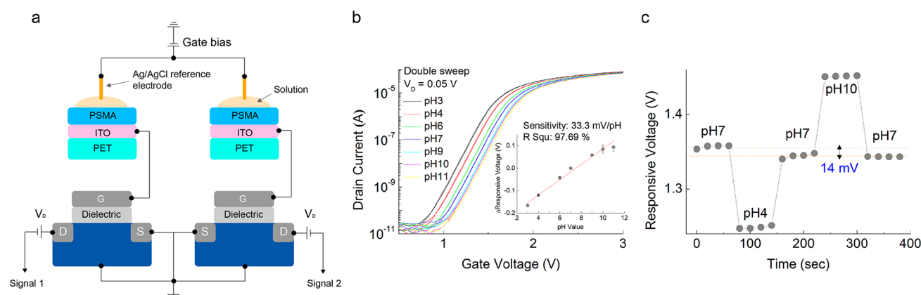
Figure 1. (a) Schematic image of the measurement system. Two different remote sensing gates were coupled to the gate of each commercial FET. (b) Representative transfer curves of FET with the remote PSMA membrane with changing pH values. The inset figure shows \Delta V_R versus pH values from an aggregate of five transfer curves. (c) Hysteresis measured through a pH loop of pH 7–4–7–10–7.
