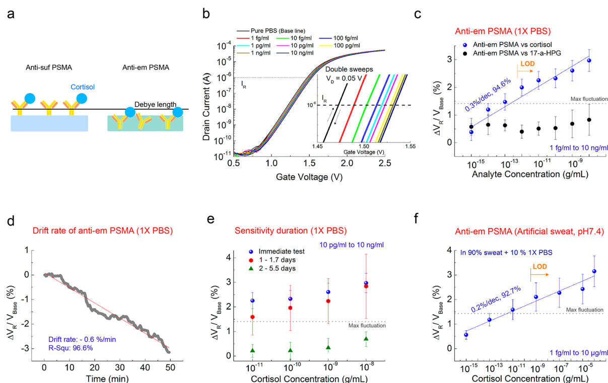
Figure 3. (a) Presumed schematic image of antibody-embedded geometric in the PSMA polymer matrix. (b) Representative transfer curves of antiem PSMA versus cortisol concentration in 1X PBS. Inset: Close-up transfer curves. (c) \Delta V_R response of antiem PSMA in terms of the cortisol and 17- \alpha -HPG concentration V_R in a 1X PBS solution. \Delta V_R increases by 0.3% with increasing cortisol over eight samples of antiem PSMA. Random signal in terms of 17- \alpha -HPG over four samples of antiem PSMA. (d) Drift properties of antiem PSMA in 1X PBS over 50 min after stabilization. A negative slope was obtained like that of Figure 2d. (e) Cortisol sensitivity of antiem PSMA as a function of days stored, in a range of cortisol from 10 pg/mL to 10 ng/mL (10 and 6 samples for immediate and stored samples, respectively). Random signals appeared for six samples 2 days after storage. (f) Cortisol sensitivity of antiem PSMA in artificial sweat with pH 7.4 in a range from 1 fg/mL to 100 \mu g/mL for five samples. 10% 1X PBS was added to the artificial sweat. Three other samples gave little or no response.
