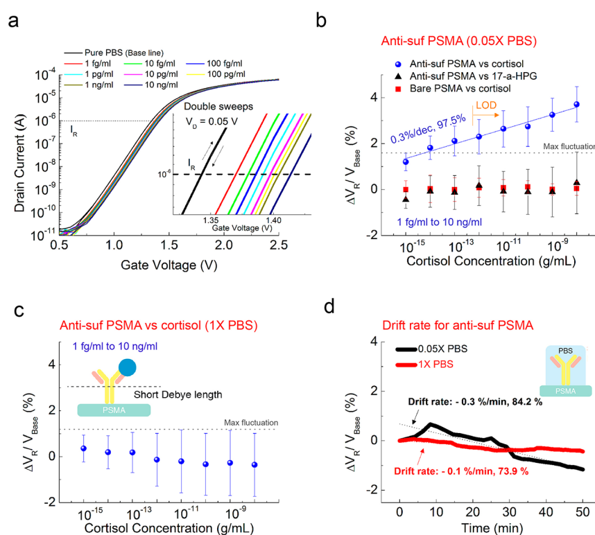
Figure 2. (a) Representative transfer curves of antisuf PSMA versus cortisol concentration in 0.05X PBS. Inset: Close-up transfer curves. (b) \Delta V_R response of antisuf PSMA in terms of cortisol and 17- \alpha -HPG concentrations in 0.05X PBS. The \Delta V_R response of cortisol on bare PSMA is compared. Mean \Delta V_R increase by 0.3% for every 10-fold increase in the cortisol concentration for five samples. Random signals for cortisol were observed in the bare PSMA for four samples. Also, no sensitivity for 17- \alpha -HPG is obtained by antisuf PSMA for three samples. (c) \Delta V_R of antisuf PSMA versus different concentrations of cortisol in a 1X PBS solution over three samples. (d) Drift rate of antisuf PSMA measured in 1X and 0.05X PBS by repeating the transfer curve for 50 min after stabilization. In both cases, the drift had a negative slope.
