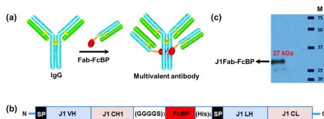
Figure 1. (a) Schematic representation of multivalent antibody production. Fab-FcBP is ligated to the Fc region of IgG to generate a multivalent antibody. (b) Schematic diagram of the phagemid vector in which the Fab fragment of the J1 monoclonal antibody is cloned. (c) Western blot analysis of J1Fab-FcBP.
