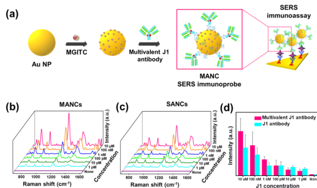
Figure 3. (a) Schematic illustration of MANC preparation for J1 peptide detection. In the presence of J1, MANC-on-nanoplate structures are constructed, and SERS signals of MGITC are observed. (b) SERS spectra of MGITC obtained from MANC-on-nanoplate structures by varying the concentration of J1. (c) SERS spectra of MGITC obtained from SANC-on-nanoplate structures with varying J1 concentrations. (d) Plot of band intensity at 1,175\text{ cm}^{-1} versus the concentration of J1. Magenta and cyan bars were obtained using MANCs and SANCs, respectively. Data represent the mean plus standard deviation of eight measurements.
