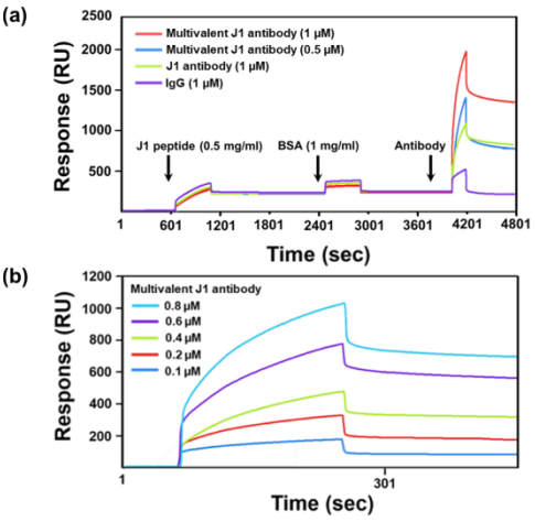
Figure 2. (a) Antigen-binding abilities of the multivalent J1 antibody (0.5 and 1 \mu\text{M} ), standard J1 antibody (1 \mu\text{M} ), and IgG (1 \mu\text{M} ) using J1 peptide-coated SPR chips. RU values were obtained from three independent experiments. (b) Antigen-binding ability of the multivalent J1 antibody (0.1, 0.2, 0.4, 0.6, and 0.8 \mu\text{M} ) using J1 peptide-coated SPR chips.
