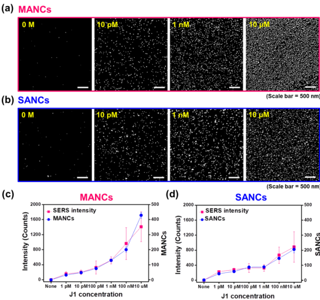
Figure 4. (a) SEM images of MANC-on-nanoplate structures with varying J1 concentrations. (b) SEM images of SANC-on-nanoplate structures with varying J1 concentrations. (c) SERS intensity and number of MANCs on nanoplates ( 1\ \mu\text{m} \times 1\ \mu\text{m} ) as a function of J1 peptide concentration. (d) SERS intensity and number of SANCs on nanoplates ( 1\ \mu\text{m} \times 1\ \mu\text{m} ) as a function of J1 peptide concentration.
