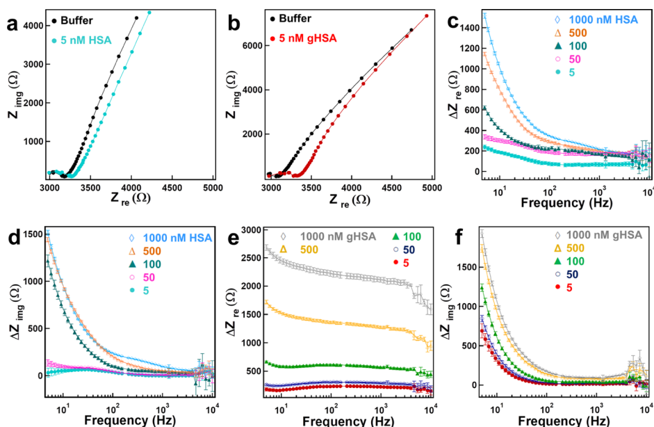
Figure 3. EIS detection of HSA and gHSA. (a,b) Nyquist plots for PEDOT–IDA biosensors in solutions of buffer (black) and 5 nM HSA (blue) or gHSA (red). (c–f) \Delta Z_{re} and \Delta Z_{im} plots vs frequency for PEDOT–IDA biosensors exposed to varying concentrations of HSA (c,d) and gHSA (e,f), where \Delta Z is defined as Z_{HSA} - Z_{buffer} . Error bars are defined as a propagated error from the standard deviation, \pm 1\sigma , for five consecutive EIS measurements.
