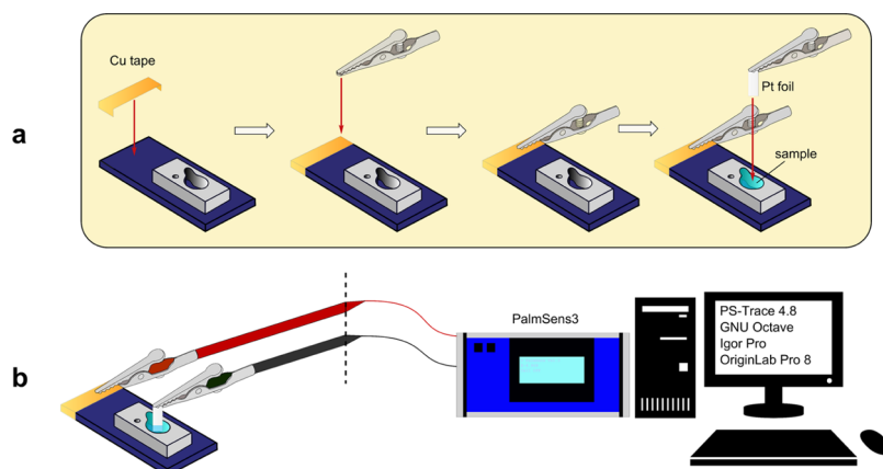
Figure 7. Preparation of the biosensor for measurements. (a) Electrical contacts to the prepared devices are made with copper tape, platinum foil (as the counter electrode), and alligator pins. (b) Measurements were performed using a PalmSens3 analyzer controlled by PSTrace 4.8. Data were processed with GNU Octave, Igor Pro, and OriginLab Pro 8.
