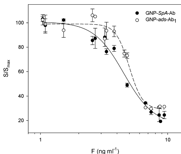
Figure 4. Correlation curves between normalized signals ( S/S_{\max} ) provided by two LFDs for 13 human salivary samples and the cortisol concentration as measured by a reference ELISA. The two LFDs varied for the probe that was either prepared by the SpA-mediated attachment and by direct adsorption of anticortisol antibodies to GNPs. S_{\max} was estimated from interpolation of experimental values by the 4-parameter equation.
