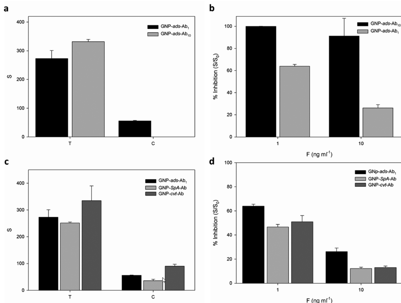
Figure 3. Signals ( S ) generated at the test (T) and control (C) lines by probes prepared: (a) by adsorbing 1 (GNP-ads-Ab 1 ) and 10 \mu g (GNP-ads-Ab 10 ) of anticortisol antibody to 1 mL of GNP, and (c) by mediated coupling via chemical (GNP-cvt-Ab) or biochemical (GNP-SpA-Ab) layers. The sensitivity of the LFIA employing the different probes was estimated by applying standard solutions of cortisol and measuring the corresponding inhibition rate (b, d).
