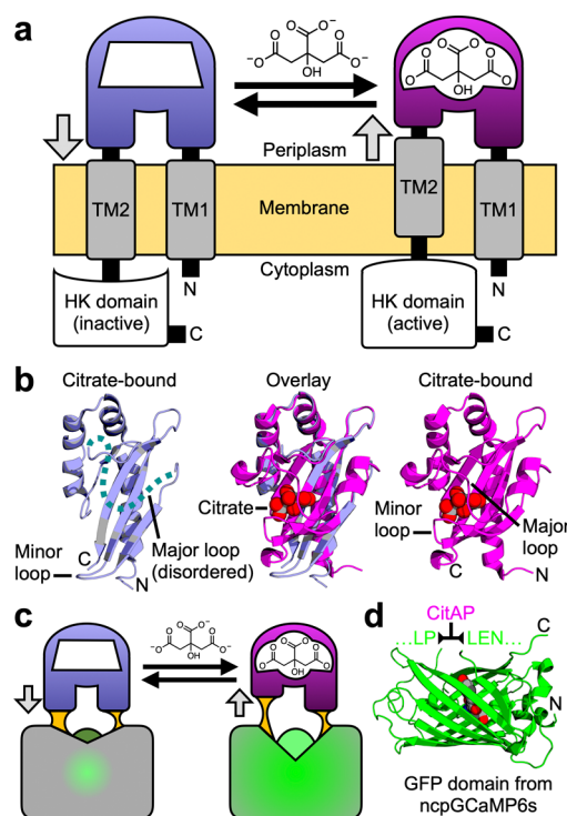
Figure 1. Rationale for the design of a single-FP-based citrate biosensor. (a) Schematic representation of Klebsiella pneumoniae SHK CitA, which is composed of a periplasmic citrate-binding domain (CitAP; light blue, unbound; magenta, bound), connected to transmembrane helices at both its N- (transmembrane helix 1, TM1) and C-termini (transmembrane helix 2, TM2). TM2 is, in turn, connected to an intracellular HK catalytic domain. 26 (b) The structures of citrate-free CitAP (left; light blue; PDB ID 2V9A), 25 citrate-bound CitAP (right; magenta; PDB ID 2J80), 25 and a superposition of the citrate-free and -bound structures (middle). (c) We hypothesized that the piston-type conformational motion at the CitAP termini could be communicated to GFP to allosterically control the chromophore environment and its fluorescent brightness. In this way, the CitAP domain could serve as the basis of construction of a genetically encoded citrate biosensor. (d) To realize this biosensor design, we inserted CitAP into GFP by replacing the CaM-RS20 domain of ncpGCaMP6s 27 with CitAP.
