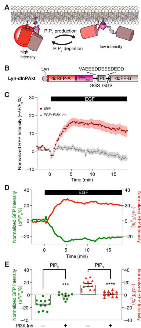
Figure 3. Development of fluorescence intensity-based reporter dInPAkt and multiplexed imaging of phosphoinositide dynamics. (A) Schematic representation of dInPAkt, where PH_{Akt} binding to membrane 3-phosphoinositides leads to an increase in distance between the two dimerization-dependent RFP monomers ddRFP-A (red, bright) and ddFP-B (dark) and a decrease in fluorescence intensity, because of the loss of ddFP heterodimerization (red, dim). Therefore, the production of 3-phosphoinositide membranes will thus lead to a decrease in red fluorescence intensity. (B) Graphic illustration of the domain structure of the Lyn-targeted dInPAkt. (C) Time course of normalized dInPAkt red fluorescence intensity in response to EGF stimulation (100 ng/mL) in Cos7 cells with (triangles, n = 9 ) or without (circles, n = 11 ) PI3K inhibitor preincubation. Images were acquired every 20 s. Shaded areas represent SEM (D) Time course of PIP_2 depletion (monitored by Lyn-dPlcR, shown in green) and production of 3-phosphoinositides (Lyn-dInPAkt, shown in red) in Cos7 cells in response to EGF. Plots shown are representative single-cell traces. Additional single-cell traces from independent experiments are shown in Figures S11 (no pretreatment) and S14 (with PI3K preinhibition) in the Supporting Information. (E) Statistical analysis of membrane PIP_2 (circles) and 3-phosphoinositide (diamonds) levels after 5 min of EGF stimulation (100 ng/mL) in Cos7 cells with (+) or without (-) PI3K preinhibition, quantified from single-cell traces in Figures S11 and S14. [Legend: (***) p < 0.001 and (****) p < 0.0001 , from Student's t -test.]
