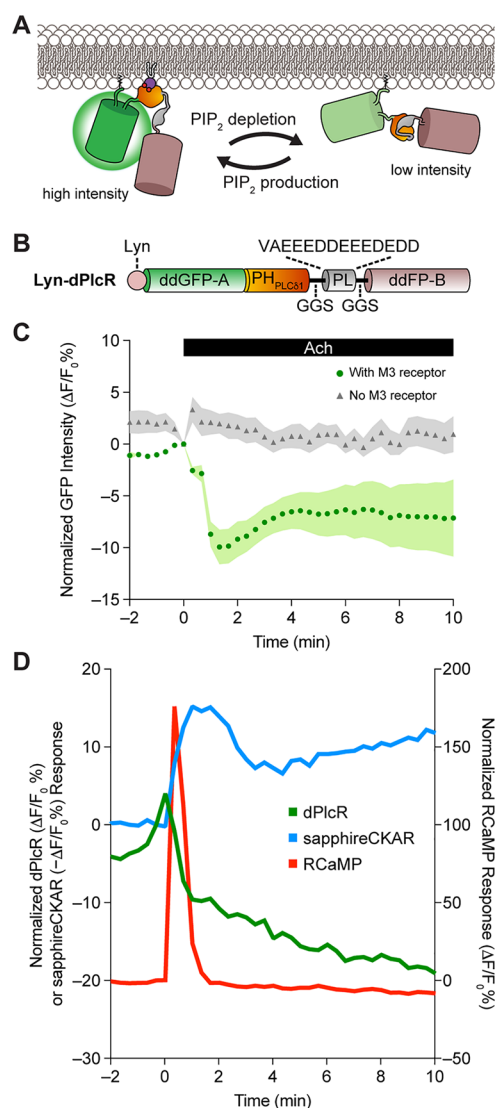
Figure 2. Development and characterization of fluorescence intensity-based PIP 2 reporter dPlcR. (A) Schematic representation of dPlcR, where PH PLCδ1 binding to membrane PIP 2 leads to a decrease in the distance between the two dimerization-dependent GFP monomers ddGFP-A (green, dim) and ddFP-B (dark) and an increase in fluorescence intensity, as a result of ddFP heterodimerization (green, bright). Depletion of membrane PIP 2 will thus lead to decreased green fluorescence intensity. (B) Graphic illustration of the domain structure of plasma membrane-targeted Lyn-dPlcR. (C) Time course of normalized Lyn-dPlcR green fluorescence intensity in Cos7 cells with (circles, n = 8) or without (triangles, n = 8) G q -coupled M 3 receptor co-expression upon acetylcholine (10 μM) stimulation at t = 0 min. Images were acquired every 20 s. Shaded areas represent SEM. Single-cell traces co-monitored with the Ca 2+ indicator RCaMP are shown in Figures S6 and S7 in the Supporting Information. (D) Time course of PIP 2 depletion (monitored by Lyn-dPlcR in green), intracellular Ca 2+ influx (RCaMP in red), and PKC activity (sapphireCKAR in blue) in M 3 receptor-expressing Cos7 cells upon acetylcholine (ACh, 10 μM) addition at t = 0 min. Plots show representative traces from a single cell. Additional single-cell traces from independent experiments are shown in Figure S8 in the Supporting Information ( n = 5), and responses from cells without M 3 receptor are shown in Figure S9 in the Supporting Information ( n = 9) as a negative control.
