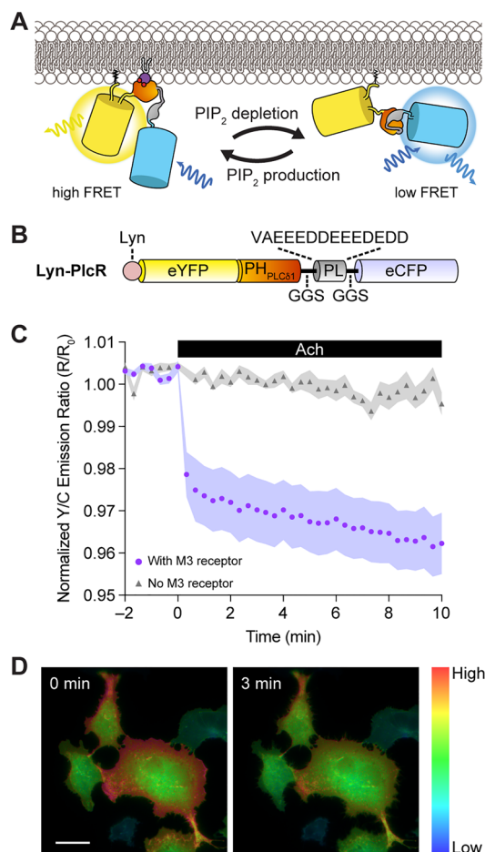
Figure 1. Development and characterization of FRET-based \text{PIP}_2 reporter PlcR. (A) Schematic representation of phospholipase \text{C}\delta 1 ( \text{PLC}\delta 1 )-based \text{PIP}_2 reporter, PlcR. A negatively charged pseudo-ligand (PL) and \text{PIP}_2 compete for binding to the PH domain of \text{PLC}\delta 1 ( \text{PH}_{\text{PLC}\delta 1} ), resulting in a conformational change upon \text{PIP}_2 depletion, where the reporter adopts a low FRET efficiency conformation between the two fluorescent proteins, enhanced Yellow Fluorescent Protein (eYFP) and enhanced Cyan Fluorescent Protein (eCFP). (B) Graphic illustration of the domain structure of plasma membrane-targeted Lyn-PlcR. (C) Time course of the normalized yellow-over-cyan (Y/C) emission ratio in Cos7 cells expressing Lyn-PlcR with (circles, n = 12 ) or without (triangles, n = 8 ) co-expression of the \text{G}_q -coupled \text{M}_3 receptor upon acetylcholine (Ach, 10 \mu\text{M} ) stimulation at t = 0 min. Images were acquired every 20 s. Shaded areas represent SEM. Single-cell traces co-monitored with the \text{Ca}^{2+} indicator RCaMP are shown in Figures S3 and S4. (D) Pseudo-color images showing the FRET ratio changes in Cos7 cells expressing Lyn-PlcR before and after acetylcholine stimulation, where warmer colors indicate high plasma membrane \text{PIP}_2 levels and cooler colors indicate low \text{PIP}_2 . Scale bar = 10 \mu\text{m} .
