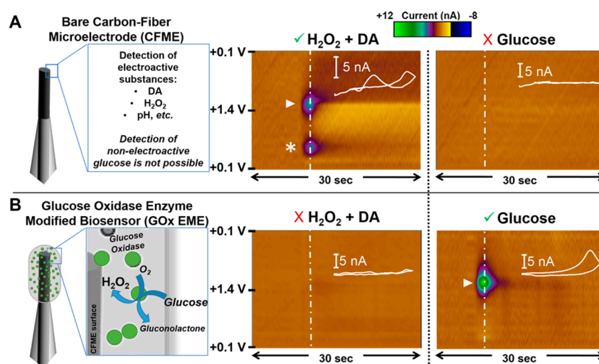
Figure 2. Voltammetric response of carbon-fiber microelectrodes to glucose, dopamine and H 2 O 2 . (A) Left: Schematic representation of a bare CFME. Representative color plots depict current collected in response to the same solutions using a voltammetric waveform from +0.1 to +1.4 V. 41 A mixture of 1000 nM DA (asterisk) and 50 μM H 2 O 2 (triangle) is detected (middle), but the detection of nonelectroactive glucose (0.8 mM) is precluded (right). (B) Left: Schematic of the GOx EME. Right: Representative color plots demonstrate the detection of glucose (triangle, indicated by the oxidation of enzymatically generated H 2 O 2 ). However, there is insufficient sensitivity for the detection of physiologically relevant concentrations of H 2 O 2 and DA (middle panel).
