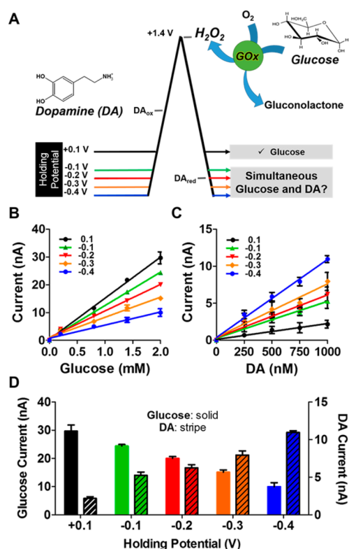
Figure 3. Systematic characterization of holding potential. (A) Investigation of a series of waveforms for the simultaneous voltammetric detection of glucose and DA with a GOx EME. (B) Glucose (0.2–2.0 mM) and (C) DA (250–1000 nM) calibration plots collected with the waveforms shown in (A). (D) The current collected in response to a sample containing 2.0 mM glucose and 1000 nM DA (note respective scales on left and right y-axes) is dependent on the holding potential applied between voltammetric scans. A -0.2 V holding potential provides a compromise that enables adequate detection of both analytes. One-way ANOVA analysis demonstrated all holding potentials were significantly different than the previously employed +0.1 V holding potential (glucose: F(4,20) = 37.28 , ***p < 0.001 ; DA: F(4,20) = 70.23 , ***p < 0.001 ).
