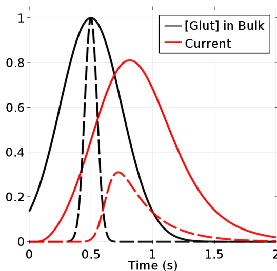
Figure 7. Glut concentration at sensor edge (relative to its maximum concentration) and observed current signal (relative to the SS current for the maximum Glut concentration). The solid curves correspond to an input pulse and output signal for a Gaussian input with \sigma = 0.25 s and C_{max} = 10 \mu\text{M} , and the dashed curves correspond to an input with \sigma = 0.05 s and C_{max} = 10 \mu\text{M} .
