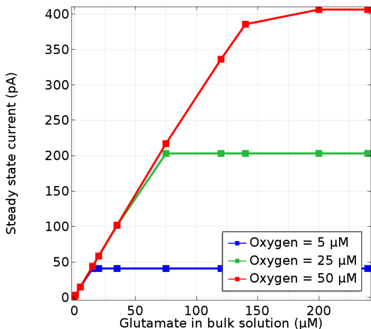
Figure 6. Steady-state response of a base-case sensor to increasing Glut concentrations over the range of O 2 concentrations typical in brain ECF.
