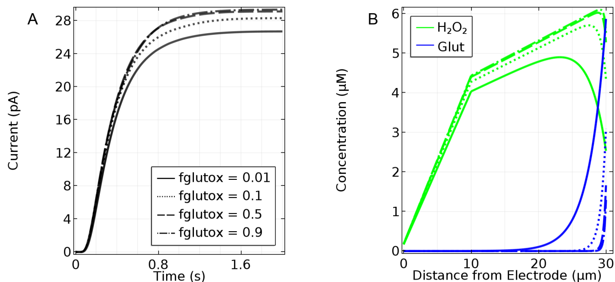
Figure 3. A. Current response to a 10- \mu M step change in Glut for sensors with 10- \mu m -thick Nafion and 20- \mu m -thick enzyme layers, where the f_{glutox} is varied from 0.01 to 0.9, and the sample O_2 concentration equals 270 \mu M . B. Corresponding plots of SS Glut and H_2O_2 concentration profiles in the Nafion and enzyme layers. Note that the outer edge of the Nafion layer is at 10 \mu m and the outer edge of the sensor is at 30 \mu m .
