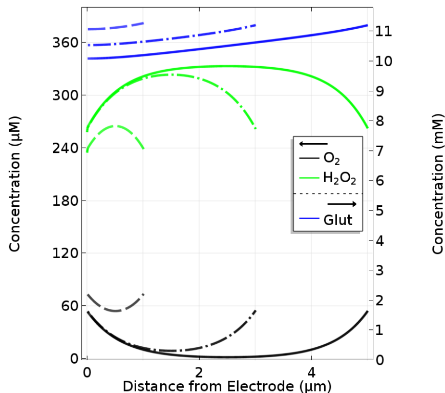
Figure 5. Concentration profiles of O 2 , H 2 O 2 , and Glut for sensors with 1, 3, or 5 μm thick enzyme coating after reaching a steady state with saturating Glut (12 mM). In all cases, f_{glutox} = 0.5 and the sample O 2 concentration equals 270 μM.
