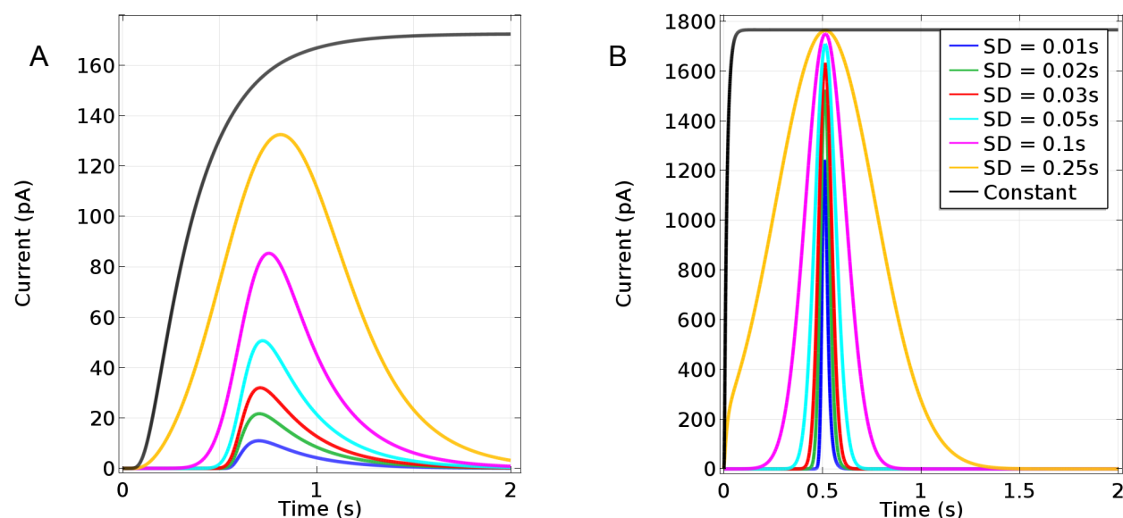
Figure 8. A. Modeled base-case sensor response to a single pulsed Glut concentration reaching maximum glutamate concentration ( C_{max} = 10 \mu\text{M} ) at 0.5 s and with standard deviations ranging from 0.01-0.25 s and to a step change in bulk sample Glut concentration to 10 \mu\text{M} for reference. B. Responses of a sensor with 1 \mu\text{m} Nafion and 3 \mu\text{m} enzyme layers to the same inputs.
