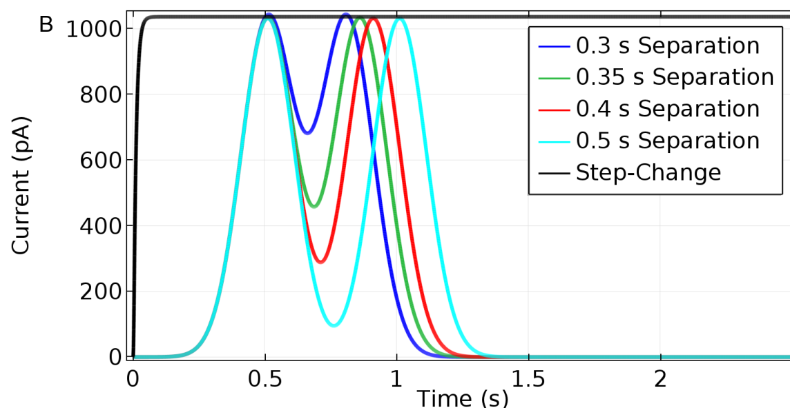
Figure 9. Sensor response to a Glut concentration step change to 10 \mu\text{M} and to two Glut pulses of \sigma = 0.1 s and C_{\text{max}} = 10 \mu\text{M} , separated by 0.3, 0.35, 0.4, and 0.5 s. A. Base-case sensor response. B. Response of a sensor with 1 \mu\text{m} Nafion and 3 \mu\text{m} enzyme layers.
