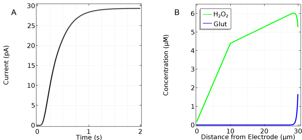
Figure 1. A. Temporal response of a base-case sensor (10 \mu\text{m} Nafion layer, 20 \mu\text{m} GlutOx layer) to a 10 \mu\text{M} step in bulk sample Glut concentration with sample \text{O}_2 concentration at 270 \mu\text{M} and B. the corresponding steady-state \text{H}_2\text{O}_2 concentration profile within the sensor layers. Note that the outer edge of the Nafion layer is at 10 \mu\text{m} and the outer edge of the sensor is at 30 \mu\text{m} .
