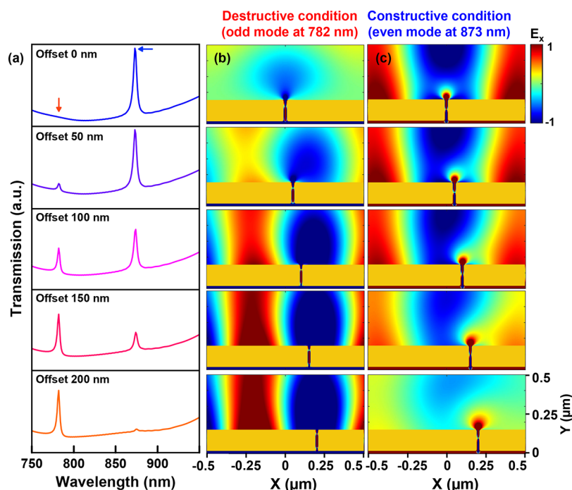
Figure 2. Split-trench resonance tuning. (a) Transmission spectra, simulated using the finite-difference time-domain method, for split-trench resonators with a feed gap at different positions, from 0 to 200 nm, relative to the center. (b,c) Spatial distributions of the E_x field component in the corresponding trench resonators for wavelengths of (b) 782 nm ( n = 9 ) and (c) 873 nm ( n = 8 ). Column (b) shows the appearance of a forbidden mode at the destructive-interference condition when the geometrical symmetry is broken. Column (c) shows the extinction of a resonance peak at the constructive-interference condition as the feed gap moves to the right.
