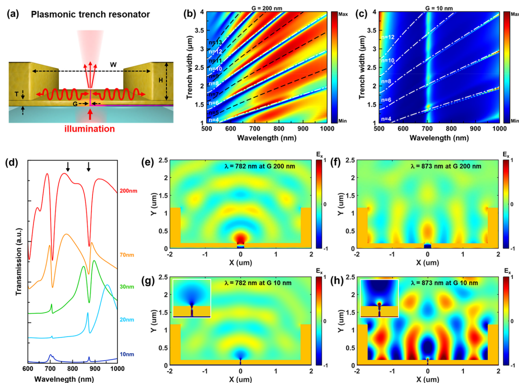
Figure 1. Split-trench resonator architecture and optical response. (a) The resonator consisting of a metal film, a feed gap, and sidewall mirrors. In the trench, surface plasmon waves excited by illuminating the subwavelength slit feed cavity resonances and create plasmonic standing waves. Calculated optical transmission spectra show complex resonances formed by the interference between surface-plasmon modes inside the trench and light transmitted directly through the slit. (b,c) Dispersion maps for trench resonators with (b) 200 nm gaps and (c) 10 nm gaps drilled in 130 nm thick gold films. White dashed lines indicate the constructive condition of the in-plane component of the electric field, E_x , for even diffraction orders, n (see eq 2), and black dashed lines represent the destructive condition for odd orders. (d) Transmission spectra, simulated using the finite-difference time-domain (FDTD) method, for trench resonators of width W = 3.4\text{ }\mu\text{m} with increasing gap sizes. (e,f) Spatial distributions of E_x at diffraction orders (e) n = 9 and (f) n = 8 in the trench resonator with a 200 nm gap. (g,h) Spatial profiles of E_x at the same diffraction orders but with a 10 nm gap.
