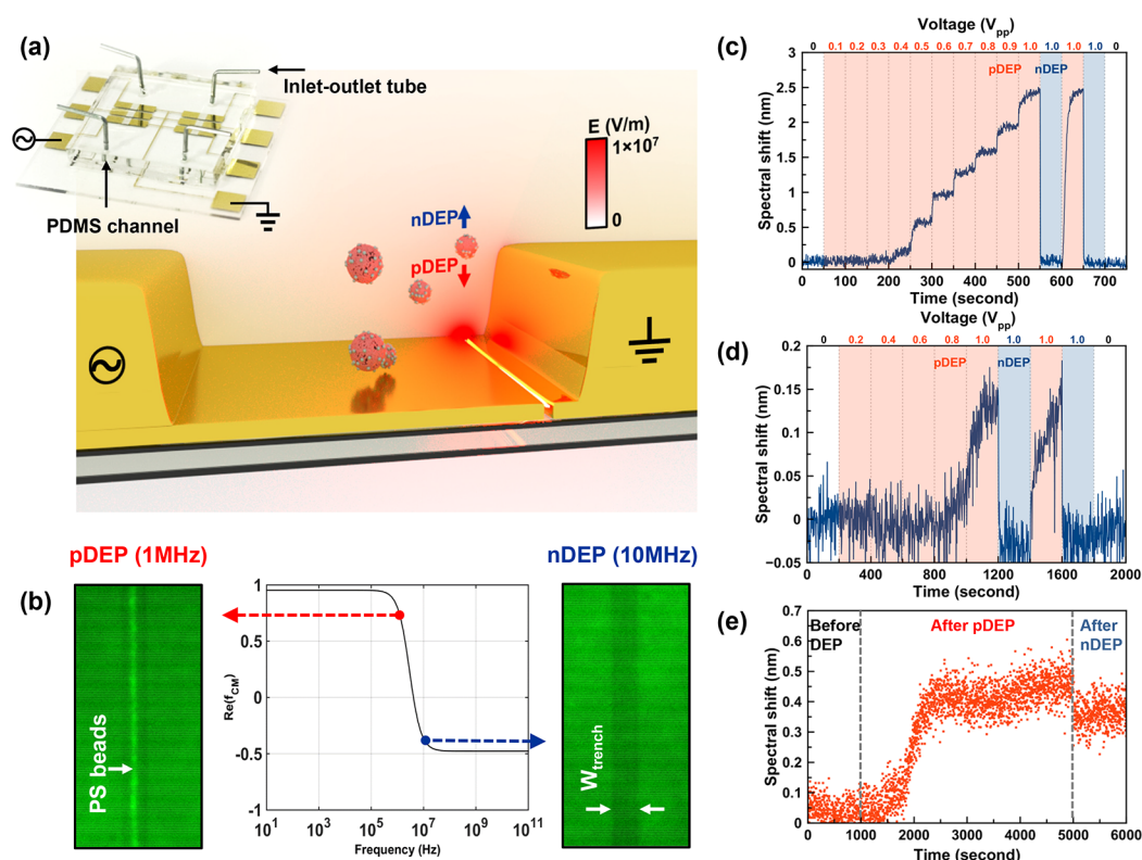
Figure 5. DEP-enhanced plasmonic sensing. (a) Conceptual illustration of DEP forces attracting biomolecules toward an RF-biased slit (pDEP) or repelling them away (nDEP). Overlaid is the simulated electric field of a 1 V bias applied across a 10 nm gap. The inset contains a photograph of a six-device chip with PDMS microfluidics. (b) The real part of the Clausius–Mossotti factor, \Re[f_{CM}(\omega)] , for suspended polystyrene (PS) beads (measured conductivity: 0.28 mS/m) as a function of RF frequency. Side panels contain fluorescence images of 190 nm PS beads attracted to (1 MHz) and repelled from (10 MHz) the nanogap. (c) Optical transmission resonance shifts as a function of applied voltage ( V_{pp} from 0 to 1 V) and time as 190 nm PS beads are trapped. (d) Same as (c) except with 30 nm PS beads. (e) Spectral shift as bovine serum albumin molecules (10 pM concentration) are trapped with a positive DEP bias of 5 V and 1 kHz frequency. After 5000 s, a 10 MHz frequency is applied and the DEP becomes negative.
