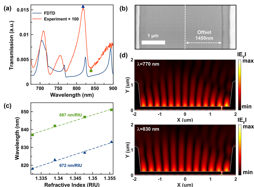
Figure 4. Optical characterization. (a) Optical transmission spectrum from an asymmetric trench-resonator biosensor immersed in water. A computer-simulated spectrum (blue solid line) is compared with the experimentally measured one (red). (b) SEM image of the asymmetric trench nanogap resonator. The offset of the slit from the center of the trench resonator is 1450 nm. (c) Measurements of bulk refractive index sensitivity. (d) Simulated electric field distributions for the asymmetric trench resonator in water at the wavelengths of 770 nm (top) and 830 nm (bottom).
