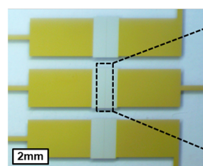
Figure 3. Device fabrication via atomic layer lithography. (a) High-throughput batch fabrication of centimeter-long arrays of trench resonators using atomic layer deposition and photolithography. (b) Patterning a single nanogap structure and integration of sidewalls. (c) Optical-microscope image of a chip including multiple trench resonators. (d) Top-down scanning electron micrograph (SEM) of trench resonator. (e) Cross-sectional SEM of trench resonator.
