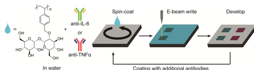
Figure 2. Direct electron beam patterning process for generating antibody patterns. An aqueous solution containing PolyProtek, ascorbic acid, and target antibody is spin-coated on a PEG-silane-coated substrate and subsequently patterned by electron beam lithography. Non-cross-linked areas are washed away. Multicomponent antibody patterns can be generated by spin-coating a new layer with a different antibody, alignment and subsequent e-beam patterning, and rinsing.
