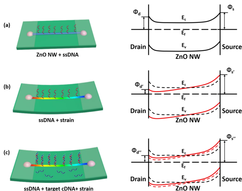
Figure 5. Schematic band diagrams of the ZnO NW DNA sensor under different conditions: (a) unstrained, (b) compressively strained and functionalized with ssDNA but without the target DNA, (c) compressively strained, functionalized with ssDNA, and hybridized with the target DNA.
