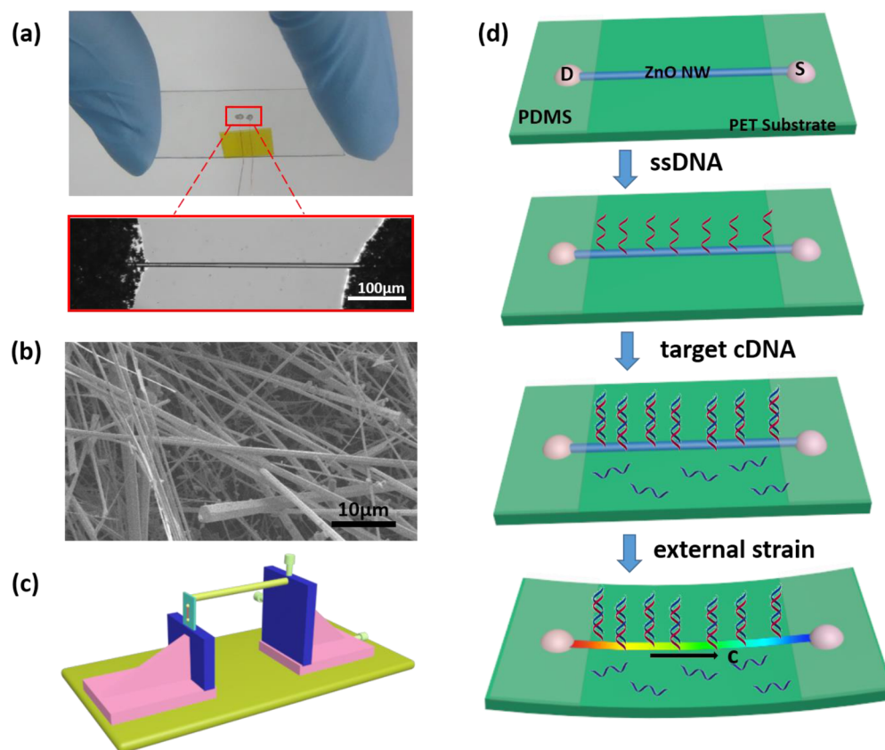
Figure 1. (a) Digital image and optical microscopy image of the ZnO NW DNA sensor. (b) SEM image of the as-synthesized ZnO NWs. (c) Schematic illustration of the experimental setup. (d) Functionalization and detection process of the ZnO NW DNA sensor under no strain and external strain.
