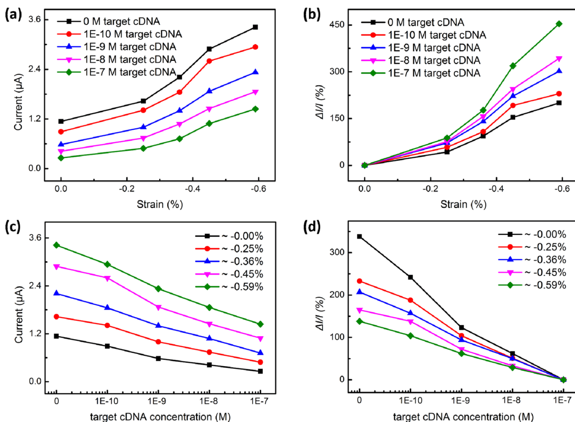
Figure 4. Enhanced performance of the ZnO NW DNA sensor by the piezotronic effect. (a, b) Absolute and relative current response of the DNA sensor to compressive strain at a fixed target cDNA concentration of 0, 1 \times 10^{-10} , 1 \times 10^{-9} , 1 \times 10^{-8} , and 1 \times 10^{-7} M, respectively. (c, d) Absolute and relative current response of the DNA sensor to target cDNA concentration at a fixed compressive strain of 0.00, -0.25 , -0.36 , -0.45 , and -0.59 , respectively.
