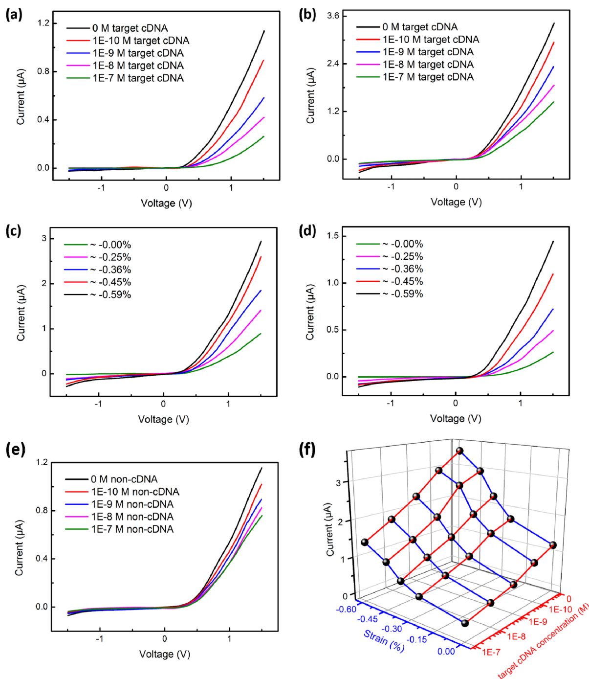
Figure 3. I – V curves of the DNA sensor under different compressive strains and DNA concentrations with a bias voltage from -1.5 to 1.5 V under (a) 0.00\% strain, (b) -0.59\% compressive strain with the target cDNA concentration ranging from 0 to 1 \times 10^{-7} M and under target cDNA concentrations of (c) 1 \times 10^{-10} M and (d) 1 \times 10^{-7} M with different compressive strains ranging from 0 to -0.59\% . (e) I – V curves of the DNA sensor under 0.00\% strain with the non-cDNA concentration from 0 M to 1 \times 10^{-7} M. (f) Current response of the DNA sensor to different compressive strains and target cDNA concentrations under a bias voltage of 1.5 V.
