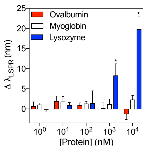
Figure 6. Dependence of LSPR shifts on protein isoelectric point (pI). Quantitative analysis of LSPR shifts of AuNS@PNM with increasing concentrations of ovalbumin (pI ~ 4.5), myoglobin (pI ~ 7.0), or hen egg white lysozyme (pI ~ 11.3) in 0.1X PBS. No significant changes in LSPR wavelength were observed upon incubation of AuNS@PNM with ovalbumin or myoglobin. However, significant shifts in LSPR wavelength were observed upon incubation of AuNS@PNM
