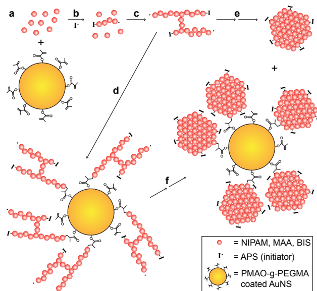
Figure 4. Schematic depiction of the process expected to lead to the AuNS@PNM flower-like architecture. (a) The monomers, N-isopropylacrylamide (NIPAM), methacrylic acid (MAA), and N,N' -methylenebisacrylamide (BIS) (pink spheres) were mixed with PMAO-g-PEGMA stabilized AuNSs (gold spheres). (b) Upon initiation with ammonium persulfate (APS, I•) at 70°C, polymer
