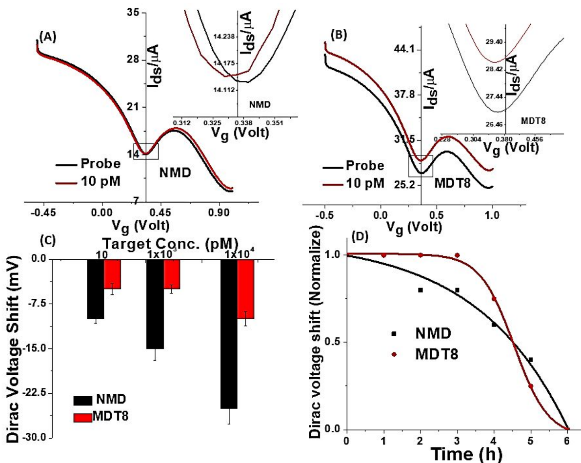
Figure 3. Direct, label-free DNA methylation profiling with GFET sensor. Concentration-dependent discrimination of methylated targets by Dirac voltage ( V_D ) shift measurements for (A) NMD, and (B) MDT8. The insets depict the regions close to the V_D minimum. (C) Concentration-dependent V_D shift data for NMD and MDT8 ( n=3 ; P \leq 0.05 ). (D) The time-dependent V_D shift was analyzed at a one-hour interval up to 6 h for NMD and MDT.
