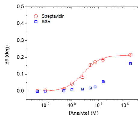
Figure 6. Angle shift vs analyte concentration for the 3MPA:11MUA biotinylated SAM. The SPR response is shown for both the affinity ligand and streptavidin (red circle) and for an interferent, BSA (blue squares).
