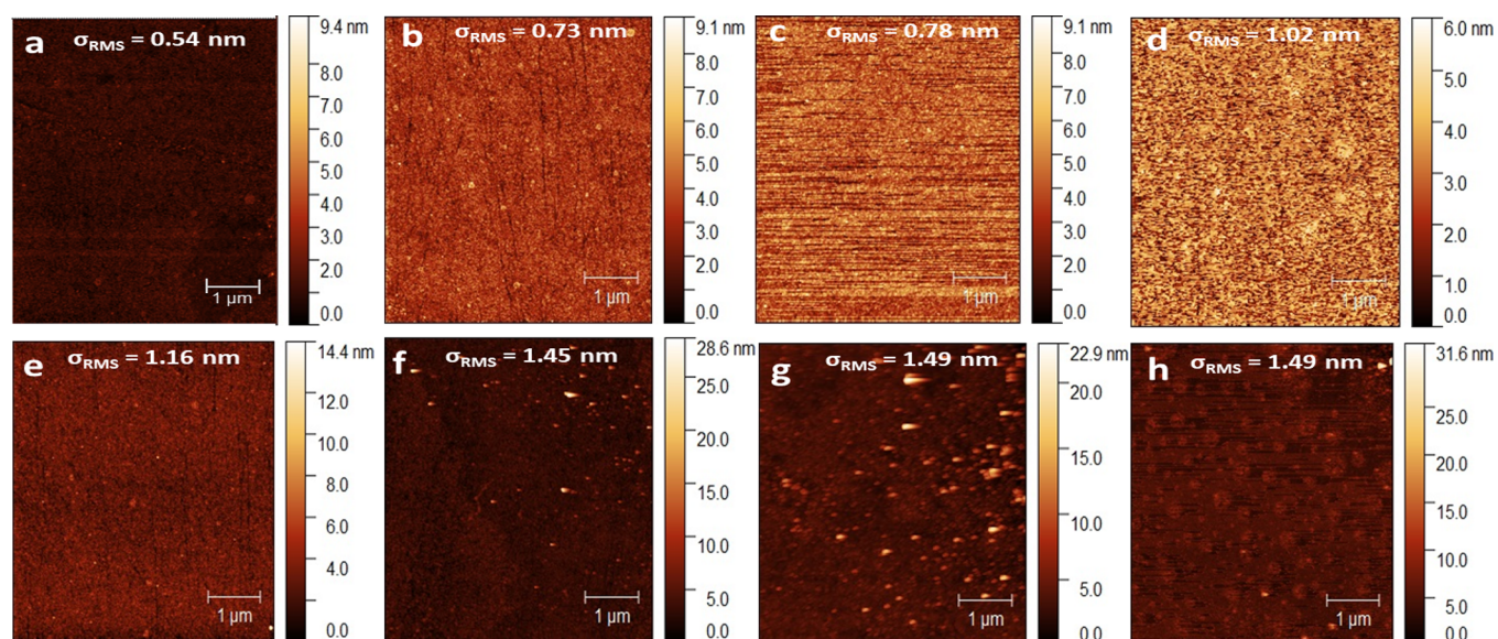
Figure 2. Representative AFM micrographs of GaAs reference surface (a), and peptide-coated GaAs at 2 (b), 5 (c), 10 (d), 25 (e), 50 (f), 75 (g), and 100 \mu\text{g/mL} (h).
