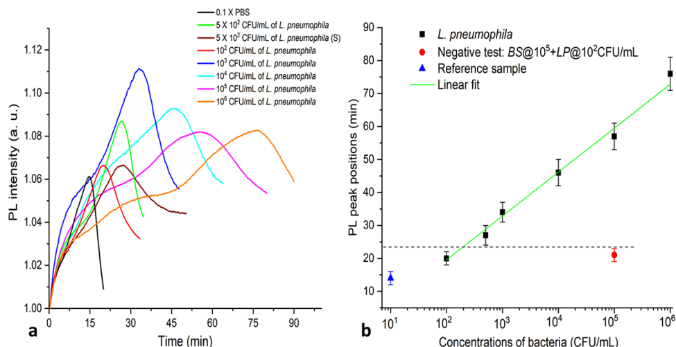
Figure 7. (a) Normalized PL intensity of AMP functionalized GaAs/AlGaAs DIP biochips (wafer D3422) exposed to different concentrations of L. pneumophila in 0.1 \times \text{PBS} , (b) PL peak positions vs different concentrations of L. pneumophila . The PL peak positions obtained for L. pneumophila are statistically different compared to either 0.1 \times \text{PBS} (reference), 10^2 CFU/mL of L. pneumophila , or the negative control test for B. subtilis + L. pneumophila exposed surfaces, as determined by the Student's t test ( n = 3 , p < 0.05 ). The dashed line highlights the biosensing resolution of the device against peak positions of the negative test and the results obtained for L. pneumophila suspension at 10^2 CFU/mL.
