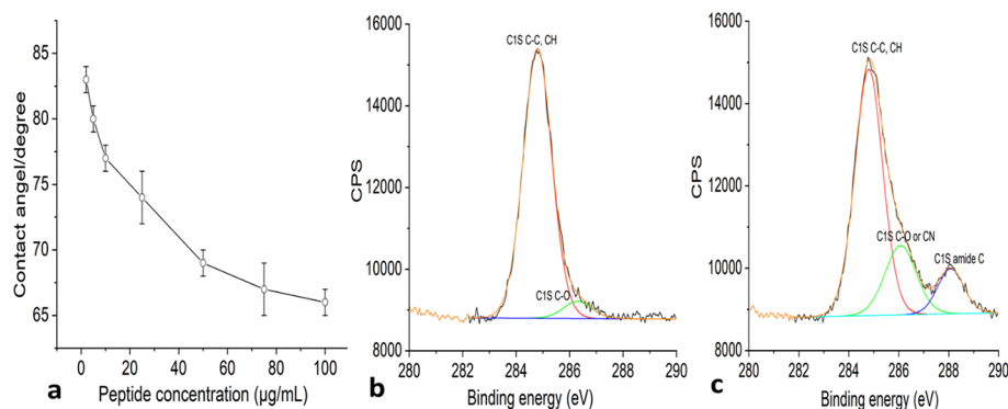
Figure 3. Water contact angle of the GaAs surface exposed to different concentrations of cysteine-modified peptides (a), and representative XPS spectra in the C 1s absorption region for the uncoated GaAs (b), and exposed to 50 \mu\text{g/mL} of a peptide solution (c). The error bars in (a) represent standard deviations of three repetitions.
