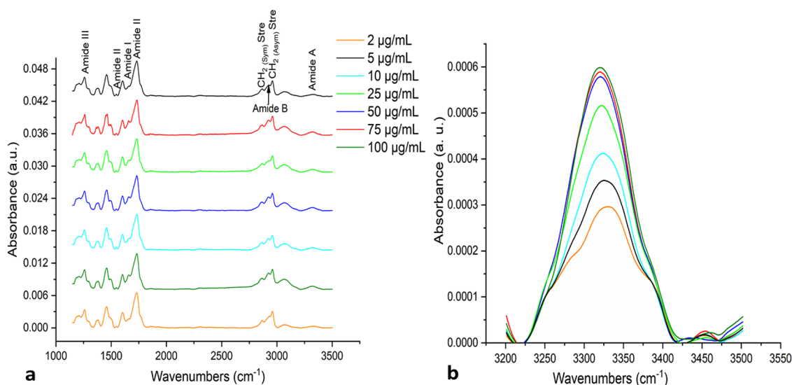
Figure 1. Representative FTIR absorbance spectra of thiol and peptide related peaks (a), and amide A absorbance spectra collected for different peptide concentrations (b).
