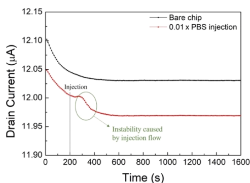
Figure 1. Transient drain current profile of a bare TFT with the microfluidic channel filled with PBS (black line). The current response profile of the TFT when the 0.01 \times PBS solution is injected to the microfluidic channel at t = 200 s (red line) is shown. The corresponding turbulence occurs at around 250–350 s.
