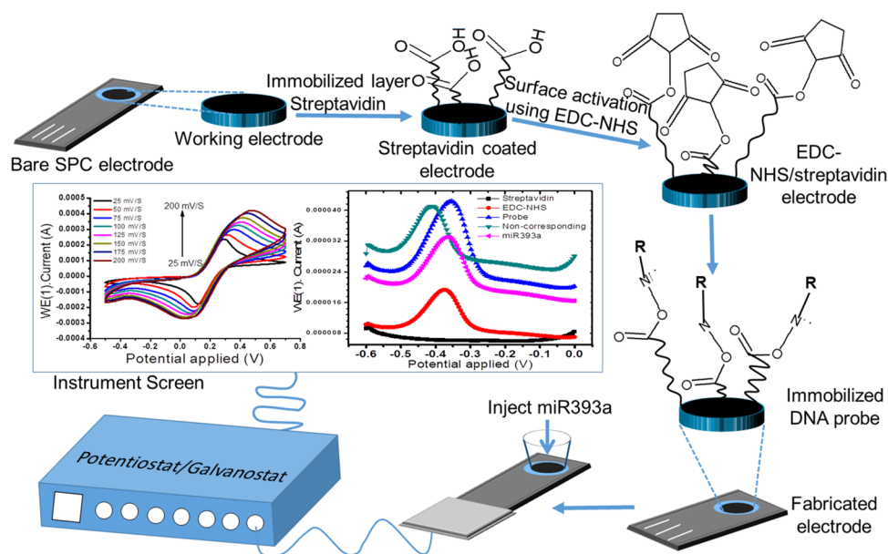
Scheme 1. Schematic Description of the Fabrication of the Probe/EDC-NHS/Streptavidin-Based Electrode Used in the Potentiostat/Galvanostat Instrument
