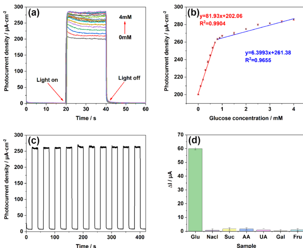
Figure 6. (a) i – t responses of TiO 2 NTs/Au/Pt toward Glu at concentrations of 0–4 mM in the supporting electrolyte of 0.1 M PBS (pH = 7.4); (b) linear calibration curve (glucose concentration vs photocurrent density); (c) stability after addition of 1 mM glucose under light conditions; and (d) anti-interference performance test performed in 0.1 M PBS (pH = 7.4) at concentrations of 0.1 mM chloride (NaCl), sucrose (Suc), ascorbic acid (AA), uric acid (UA), galactose (Gal), and fructose (Fru).
