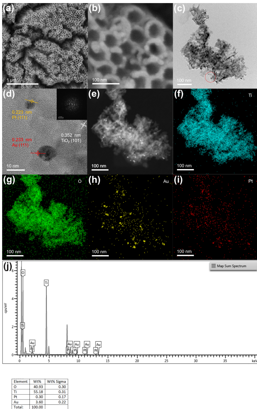
Figure 1. (b) SEM images of TiO 2 NTs/Au/Pt; (c,d) TEM and HR-TEM images of TiO 2 NTs/Au/Pt; (e–i) HAADF-STEM and mapping of Ti, O, Au, and Pt of TiO 2 NTs/Au/Pt; and (j) EDS spectra of TiO 2 NTs/Au/Pt.
