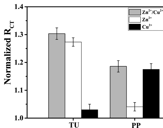
Figure 7. Histograms showing simultaneous detection of 1 nM \text{Zn}^{2+} and 1 nM \text{Cu}^{2+} in a 1:1 mixture in the presence and absence of masking agents 10 \mu\text{M} TU and 10 \mu\text{M} PP, respectively.
