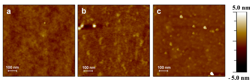
Figure 3. Atomic force microscopic images (area: 1.0\ \mu\text{m} \times 1.0\ \mu\text{m} ) recorded for (a) OT-immobilized Si/SiO 2 (OT wafer) ( \rho = 2.9\ \text{\AA} ), (b) OT wafer + 1\ \text{nM}\ \text{Zn}^{2+} solution ( \rho = 4.8\ \text{\AA} ), and (c) OT wafer + 1\ \text{nM}\ \text{Cu}^{2+} solution ( \rho = 2.0\ \text{\AA} ).
