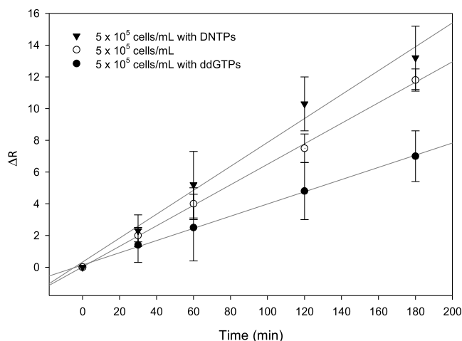
Figure 5. Changes in the charge-transfer resistance ( R ) of the Au electrode as a function of enzymatic reaction time for (▼) 5 \times 10^5 cell/mL with dNTPs, (○) 5 \times 10^5 cell/mL, and (●) 5 \times 10^5 cell/mL with ddGTP.
