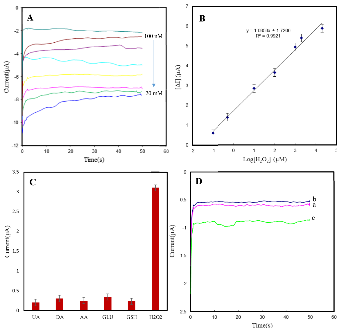
Figure 8. (A) Chronoamperometric responses of Au electrode/cerium oxide upon addition of different H_2O_2 concentrations. Applied potential: -0.5 V. (B) Logarithmic relationship between the concentrations of H_2O_2 (0.1, 0.5, 10, 100, 1000, 2000, and 20 000 \mu M ). (C) Interference studies of cerium oxide-based lab-on-a-chip device on addition of 1 mM UA, DA, AA, GLU, GSH and 0.2 mM H_2O_2 . (D) Chronoamperometric responses of Au electrode/cerium oxide for the reduction of H_2O_2 released from 10^6 PC 12 cells in 1 mL of 1 \times PBS (pH = 7.4): (a) PC12 cells, (b) AA (4 \mu M ), and (c) PC12 cells upon injection of 4 \mu M AA.
