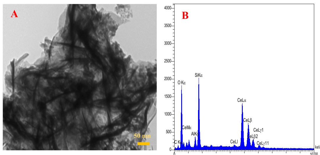
Figure 1. (A) TEM image and (B) EDS spectra of cerium oxide NSs.
