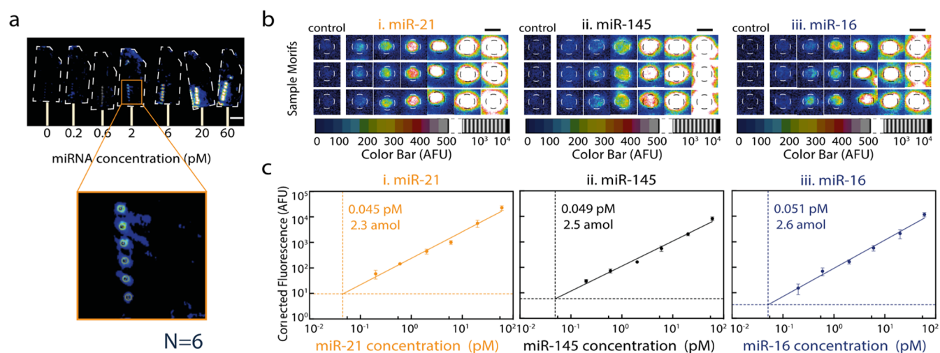
Figure 4. Investigating platform sensitivity with breast cancer-specific miRNAs. (a) Seven fibrous substrates used in the calibration curve, with a magnified view of circular regions of interest (50 \mu\text{m} radius) around each motif used in image analysis (Fiji ImageJ). (b) Fluorescence scans of three select motifs at each concentration, with high contrast color bar below (for visualization purposes). (c) Calibration curve of the corrected fluorescence vs miRNA concentration on a log–log scale, with curve fitting, and limit of detection (LOD) for miR-21, miR-145, and miR-16.
