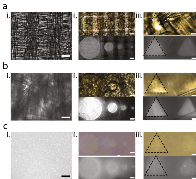
Figure 2. Patterning hydrogel motifs in fibrous substrates: (a) silk, (b) glass fiber, and (c) nitrocellulose. (i) Brightfield images of the substrate microstructure (scale bar 100 \mu\text{m} ). (ii) Brightfield (top) and fluorescence (bottom) images of circular hydrogel motifs of radii 250, 100, 50, and 25 \mu\text{m} (scale bar 100 \mu\text{m} ). (iii) Brightfield (top) and fluorescence (bottom) images of triangular motifs with dotted line outlining mask shape (scale bar 20 \mu\text{m} ).
