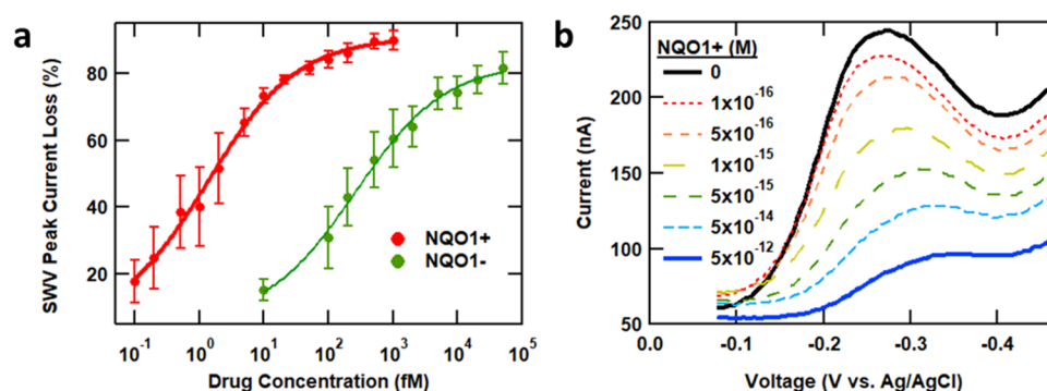
Figure 3. IB-DNQ concentration dependence. (a) Square-wave voltammetry percent peak current loss after addition of IB-DNQ to chips treated with NQO1-proficient cell lysates (NQO1+) and NQO1-deficient cells (NQO1-). Results are for three independent chips of each cell type. Error bars represent the standard error of the mean. (b) An example of the SWV signal from a single electrode in NQO1+ lysates treated with various IB-DNQ concentrations, showing a consistent signal loss.
