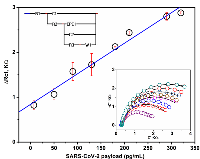
Figure 3. Calibration curve of different concentrations of SARS-CoV-2 particles ranging from 7 to 320 pg/mL. In a double-mediating electron shuttle, impedimetric responses were recorded for three successive readings. The \Delta R_{ct} ( R_{ct} captured – R_{ct} washed) was estimated by the designed Randles cell circuit from the fitted EIS signals. The correlation coefficient ( R^2 ) was 0.989, and the P -value was <0.0001 . The estimated LOD and LOQ were 57 and 157 pg/mL, respectively. R1: solution resistance, C1: capacitance of the electrode surface, R2: resistance of the CNTs/ \text{WO}_3 layer on the electrode surface, CPE1: constant phase elements of the inner layer of the electrode, C2: double-layer capacitance of polymerized meta-aminophenol (Pm-AP) on the sensor surface, R3: the resistance of the captured virus particles in the created pinholes on the VIP matrix, and W1: Warburg impedance for the diffusion of FCN/DCIP on the sensor interface.
