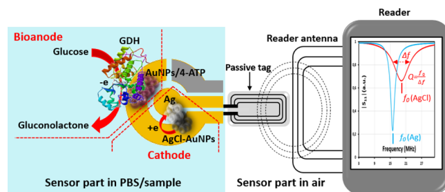
Scheme 1. Conceptual Illustration of a Battery-less and Chip-less Biosensor Tag for Wireless Measurement of Glucose in Solution a
