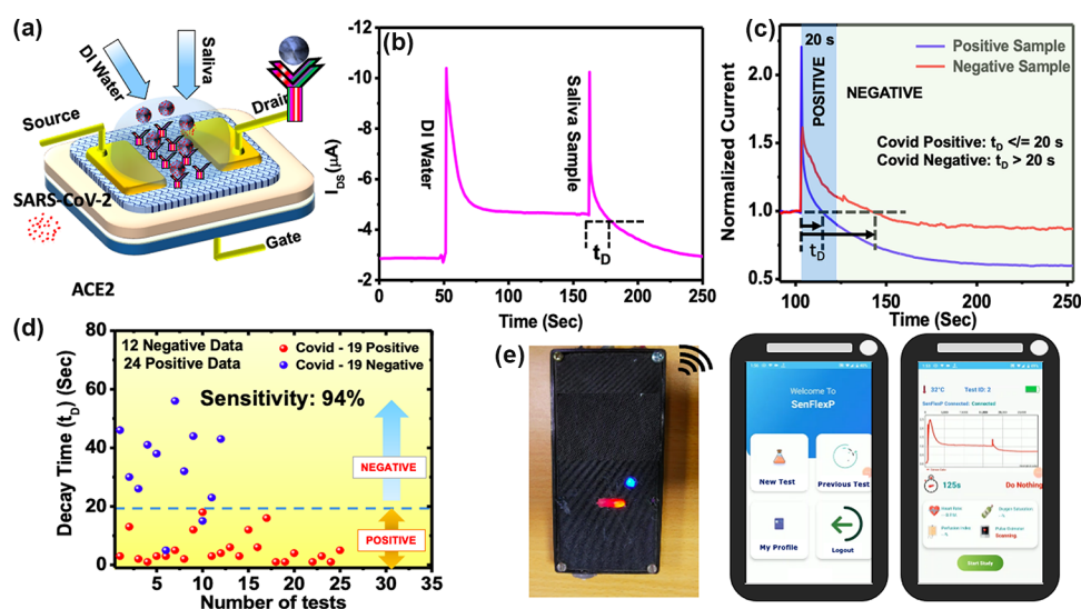
Figure 4. Detection of SARS-CoV-2 spike protein in the OFET. (a) Schematic design of the OFET indicating the steps for the detection of SARS-CoV-2. (b) Real-time variation of device current in the presence of DI water and saliva sample. (c) Variation of normalized current in the presence of COVID-positive and COVID-negative saliva samples. (d) Decay time plotted as the function of the number of tests performed. Blue and red dots represent the negative sample and positive sample, respectively. The calculated sensitivity of our device is around 94%. (e) Photograph showing the portable prototype designed for POC testing. SenFlex.P, an Android app, is developed for remotely controlling the COVID-19 test, which is connected with the prototype module via Bluetooth. The screenshot image of the SenFlex.P app during the testing is shown.
