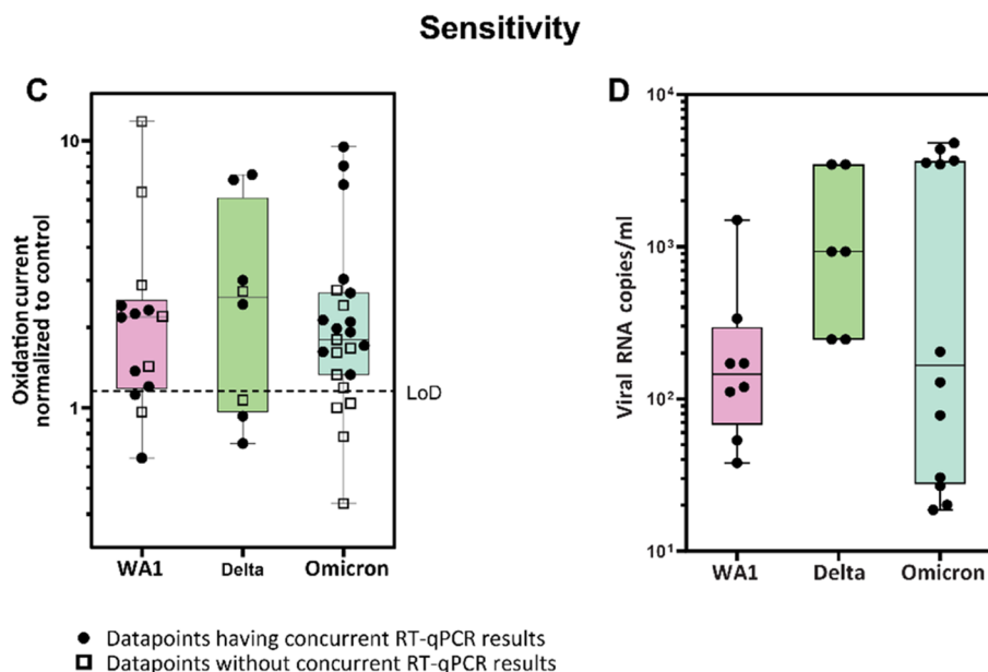
Figure 2. MIE Biosensor characteristics and EBC performance for SARS-CoV-2 detection: (A) Specificity of the MIE biosensor tested with SARS-CoV-1 and SARS-CoV-2 spike protein. (B) Biosensor sensitivity (or LoD) was evaluated by serial dilution of different SARS-CoV-2 variants. (C) Normalized oxidation current ( I_{ox} ) measured by the MIE biosensor in laboratory experiments. The horizontal dashed line denotes the limit of detection (LoD) of the system. (D) Viral RNA copies/mL determined using RT-qPCR for different aerosolized SARS-CoV-2 variants. The differences between viral RNA copies obtained for the three SARS-CoV-2 variants were statistically insignificant ( t -test, p = 0.17 ) indicating that the strain of viruses did not impact the virus collection efficiency of the breath aerosol collection device. (*Whiskers denote the range of data, and the box represents the inter-quartile range).
