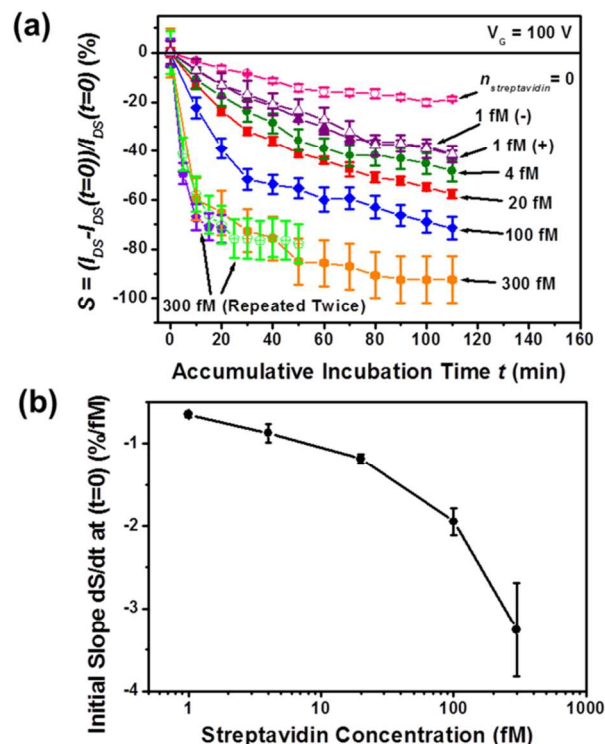
Figure 2. (a) S - t response curves measured at different streptavidin concentrations ( n_{\text{streptavidin}} = 0, 1, 4, 20, 100 , and 300 fM), which are captured from the t -dependent I_{DS} - V_G curves of a set of MoS 2 sensors; (b) plots the dS/dt - n_{\text{streptavidin}} curve extracted from the S - t response curves.
