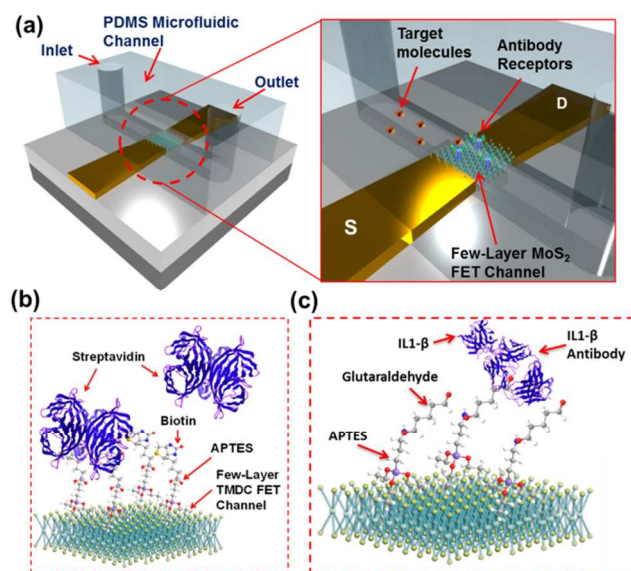
Figure 1. Experimental method: (a) illustration of a MoS 2 -based FET sensor, which is integrated with a PDMS microfluidic structure, (b) and (c) illustrations of the TMDC channels functionalized with biotin and IL-1 \beta receptors, respectively.
