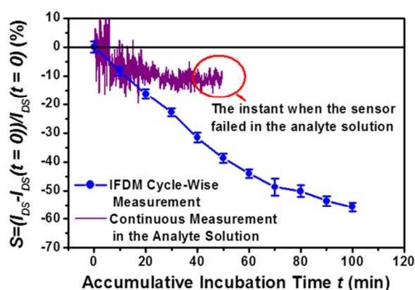
Figure 4. Comparison between the S - t response signals obtained using the IFDM cycle-wise method (solid circles) and the regular continuous detection method (solid line).
