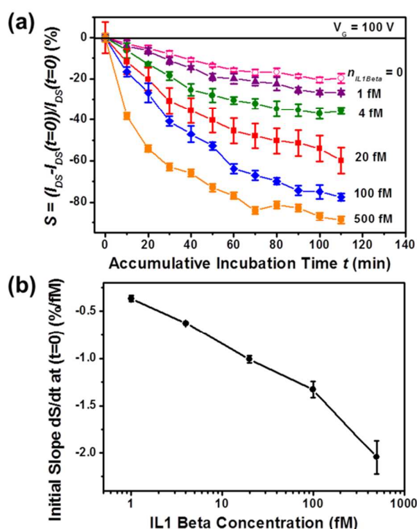
Figure 3. (a) S - t response curves measured at different IL-1 \beta concentrations ( n_{\text{IL-1}\beta} = 0, 1, 4, 20, 100 , and 500 fM), which are captured from the t -dependent I_{\text{DS}} - V_G curves; (b) plots the dS/dt - n_{\text{IL-1}\beta} curve extracted from the S - t response curves.
