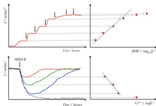
Figure 3. A: i-t curve for increasing BOD concentrations in a self-powered microbial biosensor (left), and corresponding calibration plot (right). B: i-t curve for increasing concentrations of \text{Cr}^{6+} shocks (left), and corresponding calibration plot (right).
