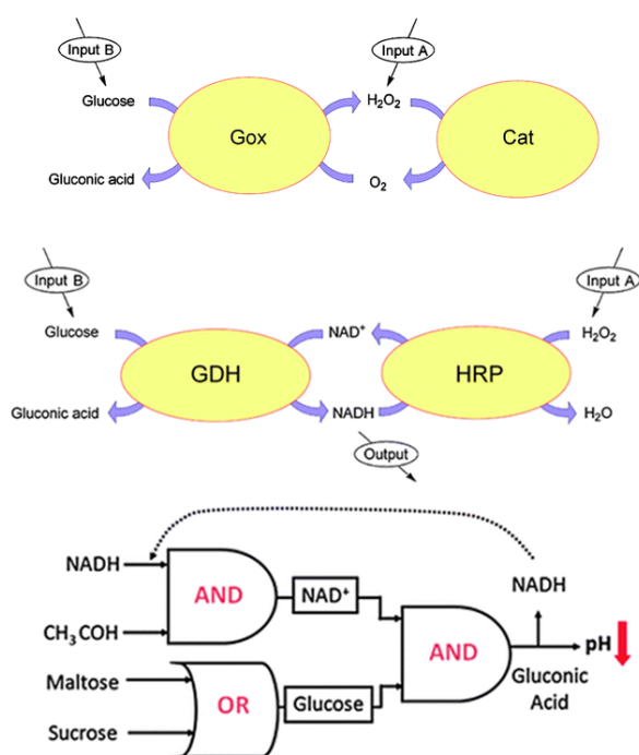
Figure 4. Examples of Enzymatic Logic Gates. (Top) AND Gate. (Middle) XOR Gate. (Bottom). Multi-gate system. Reprinted with permission from Katz, E.; Privman, V., Enzyme-based logic systems for information processing. Chem. Soc. Rev. 2010, 39, 1835-1857 86 . Copyright 2010 Royal Society of Chemistry.
