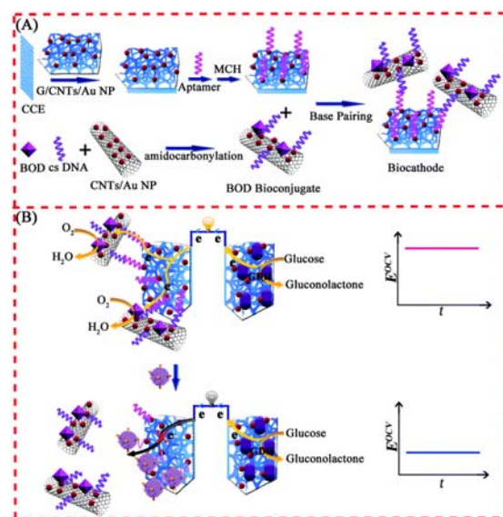
Scheme 2. Fabrication of biofuel cell and operation of the blocking scheme. Reprinted with permission from Gai, P.; Song, R.; Zhu, C.; Ji, Y.; Wang, W.; Zhang, J.-R.; Zhu, J.-J., Ultrasensitive self-powered cytosensors based on exogenous redox-free enzyme biofuel cells as point-of-care tools for early cancer diagnosis. Chem. Commun. 2015, 51, 16763–16766 52 . Copyright 2015 Royal Society of Chemistry.
