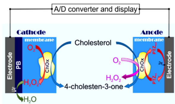
Figure 2. Schematic of a self-powered cholesterol biosensor, where PB is Prussian blue, ChOx is cholesterol oxidase, and PTZ is a phenathiazine. Reprinted in part with permission from Sekretaryova, A. N.; Beni, V.; Eriksson, M.; Karyakin, A. A.; Turner, A. P.; Vagin, M. Y., Cholesterol self-powered biosensor. Anal. Chem. 2014, 86, 9540-9547 44 .
