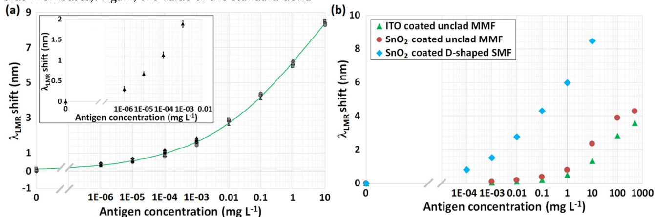
Figure 4. (a) Calibration curve of the \text{SnO}_2 -coated D-shaped SMF biosensor repeated several times and displayed together with the sigmoidal fit of the experimental points (sensor 1: grey symbols; sensor 2: dark symbols). Each cycle of measurement corresponds to a different symbol. The antigen concentration is reported in log scale. The inset shows the enlargement of the calibration curve for the lower concentration range investigated with sensor 2 (second cycle), together with the respective standard deviation for each experimental point (black error bars). (b) Comparison of the calibration curves obtained with all three kinds of LMR sensors: the ITO- (green triangles) and \text{SnO}_2 -coated (red circles) unclad MMF biosensors, and the \text{SnO}_2 -coated D-shaped SMF biosensor (sky blue rhombuses).
