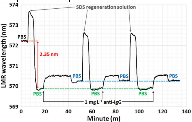
Figure 5. Regeneration test with the SDS solution repeated three times by using the ITO-coated unclad MMF biosensors (analyte concentration of 1 mg L -1 ). The red-highlighted change of the signal shows the first regeneration of the biosensing layer after the entire calibration procedure. The green-highlighted plateaux represent the value of the blank signal, while the blue-highlighted ones represent the value of the signal after the analyte injection.
