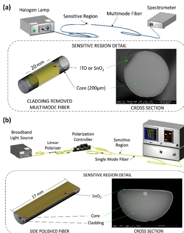
Figure 1. (a) The experimental setup for unclad MMF samples composing of a halogen lamp, a spectrometer and a 20 mm-long sensitive region realized with a thin film of ITO or SnO 2 deposited. (b) The experimental setup for D-shaped
