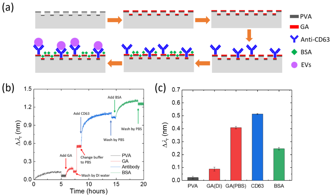
Figure 2 (a) Flow chart for the functionalization of the PC biosensor. (b) Measured wavelength shift as a function of time during the functionalization process. The black, red, blue, and green portions of the curve denote the PVA, GA, antibody, and BSA coating. (c) Resonant wavelength shift of the sensor after each step of the real-time measurement shown in (b).
