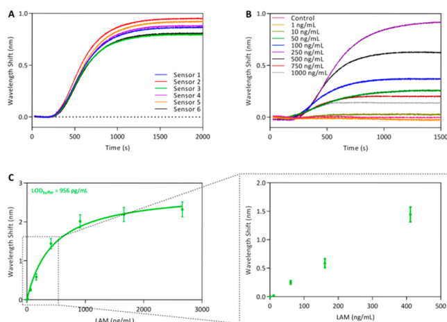
Figure 4. (A) Real-time sensogram showing the detection of 250 ng/mL LAM in buffer. (B) Sensograms showing the LAM detection at different concentrations (from 1 to 1000 ng/mL LAM) in buffer. (C) Calibration curve obtained for different LAM concentrations in buffer. Solid line corresponds to the one-site specific binding fit. All data show mean \pm SD of triplicate measurements.
