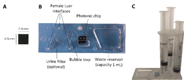
Figure 2. (A) Photonic sensor chip. (B) Microfluidic cartridge integrated with the photonic sensor chip. (C) Microfluidic cartridge employing three-syringe system.
