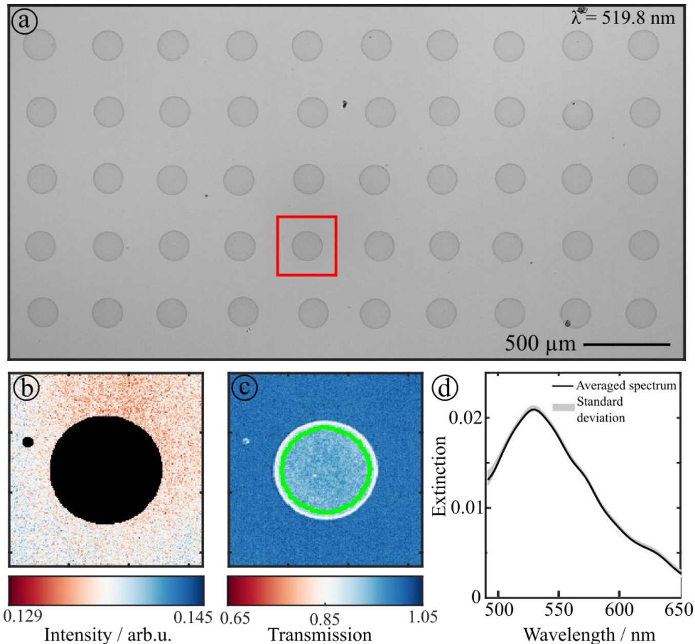
Figure 2. Image processing steps to calculate the extinction spectrum of a single nanoparticle spot. (a) Calculated bright field image of a nanoparticle spot array on glass at 519.8 nm. (b) Input area I_0(x,y,\lambda = 519.8 \text{ nm}) for the calculation of the hyperbolic surface fit used to extrapolate the background intensity under the nanoparticle spot. (c) Hyperspectral image slice after normalization by the calculated surface fit. (d) Averaged extinction spectrum of 10 subsequent measurements of the tagged nanoparticle spot. The standard deviation is plotted as grey area.
