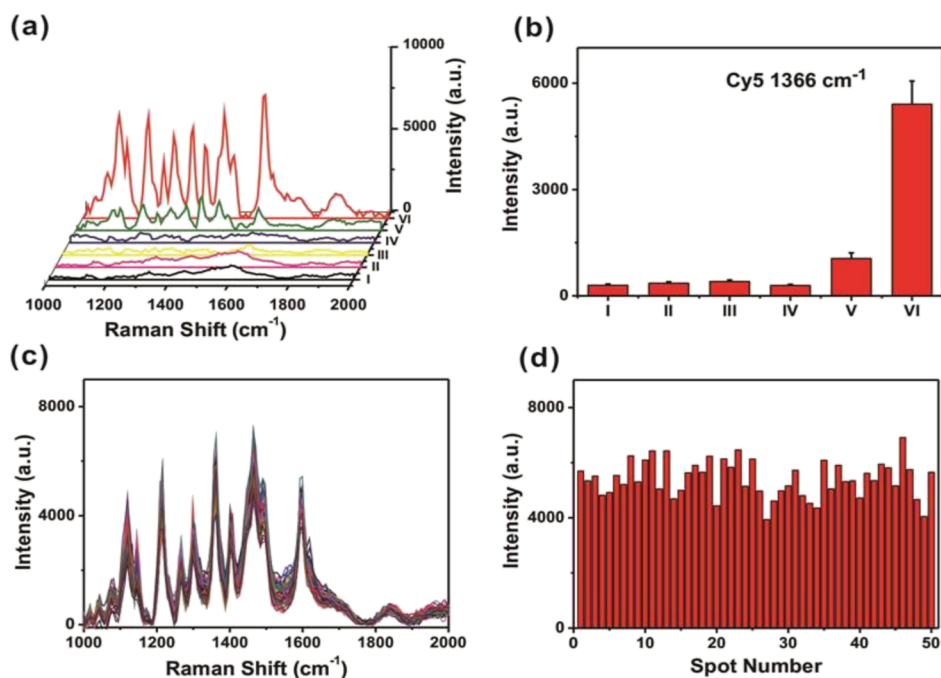
Figure 3. Validation of the ACCESS assay by SERS measurements. (a) SERS spectra of a series of control samples on the Au NPs@Si substrates immobilized with the capture DNA. (b) Intensity quantification of the SERS signals at 1366 cm -1 peak. Sample I: CCRF-CEM cell. II: aptamer. III: aptamer and probe DNA. IV: aptamer, probe DNA, and CCRF-CEM cell. V: aptamer, probe DNA, and Exo III. VI: aptamer, probe DNA, Exo III, and CCRF-CEM cell. Error bars: standard deviation from three independent assays ( n = 3 ). (c) SERS spectra of testing CCRF-CEM cell collected from 50 random spots on the Au NPs@Si substrate in a single assay. Cell number: 4 \times 10^5 per assay. (d) SERS intensity profile at 1366 cm -1 peak from the 50 random spots, corresponding to the data in (c).
