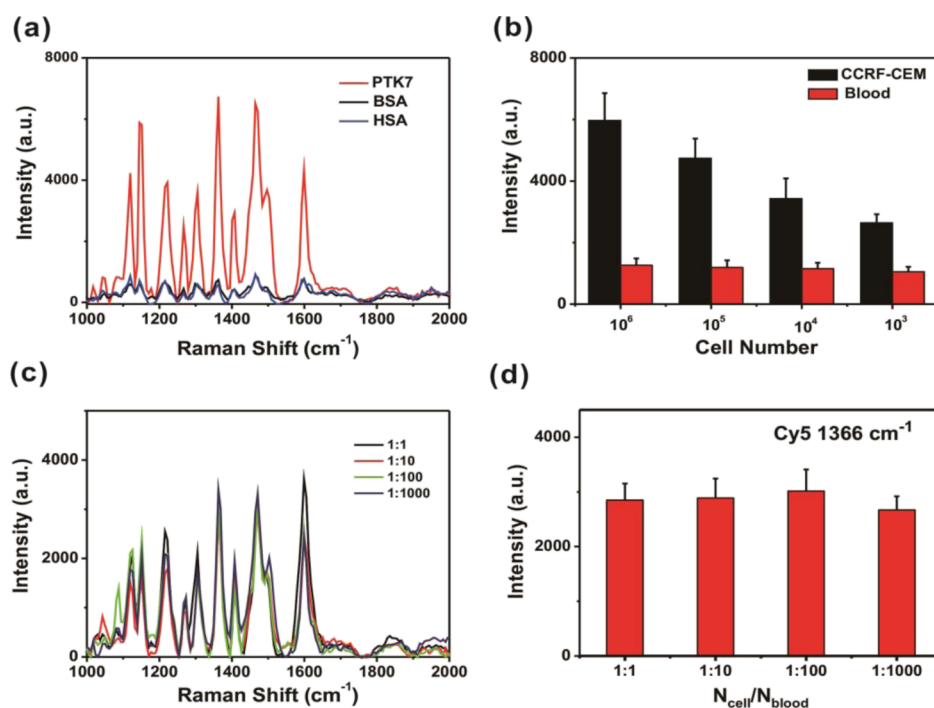
Figure 5. Specificity evaluation of ACCESS assays for the detection of PTK7. (a) SERS spectra of different protein samples on the substrates, including PTK7 and the negative controls of BSA and HAS, protein concentration: 0.1 mg mL -1 . (b) Intensity quantification of the SERS signals at 1366 cm -1 peak in testing the cell samples (CCRF-CEM cells and human blood cells separately) with different cell number per assay as specified. Error bar: standard deviation ( n = 3 ). (c) SERS spectra of testing the mixtures of CCRF-CEM cells and human blood cells in a series of dilution ratios. (d) Intensity quantification of the SERS signals at 1366 cm -1 peak in testing the mixed cell samples, corresponding to the data in (c). Error bar: standard deviation ( n = 3 ).
