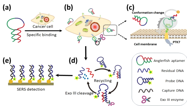
Scheme 1. Illustration of Aptamer Conformation Cooperated Enzyme-Assisted SERS (ACCESS) Technology for the Detection of PTK7 Biomarker on the Surface of Live Cells; (a) Anglerfish Aptamer; (b) Recognition between the Aptamer and PTK7 Protein; (c) Zoomed-in View of the Conformation Change due to the Recognition Event on the Cell Membrane; (d) Exo III-Assisted Cleavage of the Probe DNA, While Recycling the “Bait” DNA Segment of the Anglerfish Aptamer; (e) SERS Detection of the Residual DNA after the Cleavage. Note: The “Bait” DNA (T, Shown in Red) Segment is Not Cleaved Away from the Anglerfish Aptamer by Exo III Enzyme. For the Purpose of Simplification, Only the Exposed T Segment, Instead of the Whole Aptamer, is Illustrated in the Step of Recycling with Exo III Cleavage Reaction (d)
