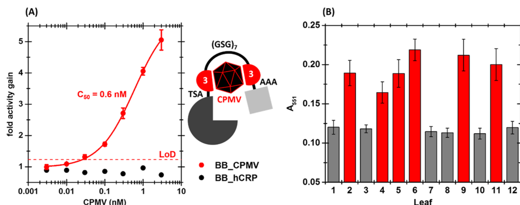
Figure 5. Plant virus (CPMV) detection. (A) Dose response of BB_CPMV to CPMV. 2 nM BB_CPMV (or BB_hCRP control) was incubated with CPMV for 10 min before 50 \mu M nitrocefin addition. Fold activity gain = \Delta A_{551} (hCRP)/ \Delta A_{551} (0 nM hCRP) read after a further 5 min. Data points are the mean of three independent measurements, and error bars indicate standard deviation from the mean. The solid line is a 4PL regression fit and the dash line indicates the LoD. (B) Detection of CPMV in infected leaves. Crude extracts of six healthy (gray) and six CPMV infected (red) leaves were prepared with the P-PER plant protein extraction kit (ThermoFisher), and 2 nM BB_CPMV was incubated with 20-fold diluted extract for 15 min before 50 \mu M nitrocefin addition. A_{551} read after a further 20 min. Data are the mean of three independent measurements, and error bars indicate standard deviation from the mean.
