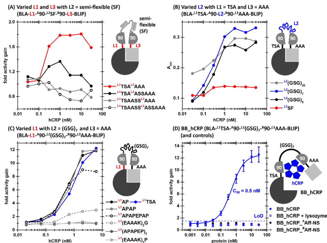
Figure 3. Re-engineering the enzyme-switch for protein (hCRP) detection. (A) Optimizing L1 and L3 (with SF L2 = (GSG) 6 A(EAAAK) 6 A-(GSG) 6 A(EAAAK) 6 A-(GSG) 6 ). 2 nM sensor incubated with hCRP for 30 min before 50 \mu M nitrocefin addition. Fold activity gain = \Delta A_{551} (hCRP)/ \Delta A_{551} (0 nM hCRP) measured after a further 30 min. (B) Optimizing L2 (with L1 = TSA, L3 = AAA). 2 nM sensor incubated with hCRP for 10 min before 50 \mu M nitrocefin addition. Read after a further 10 min and displayed as raw A_{551} to show background activity. (C) Re-optimizing L1 (with L2 = (GSG) 7 , L3 = AAA). 2 nM sensor incubated with hCRP for 10 min before 50 \mu M nitrocefin addition. Fold activity gain measured after a further 4 min. (D) Dose response of optimized hCRP sensor BB_hCRP (BLA-L1-TSA-A90-L2-(GSG) 7 -B90-L3-AAA-BLIP) and controls where Aff-hCRP90 at site A or B is replaced with a non-specific Affimer, Aff-NS (BB_hCRP A Aff-NS, BB_hCRP B Aff-NS). 2 nM sensor incubated with hCRP (or lysozyme as a control, where indicated) for 10 min before 50 \mu M nitrocefin addition. Fold activity gain read after a further 5 min. Data are the mean of triplicates in six separate repeat experiments and error bars indicate standard deviation from the mean. The solid line is a 4PL regression fit and the dash line indicates the LoD.
