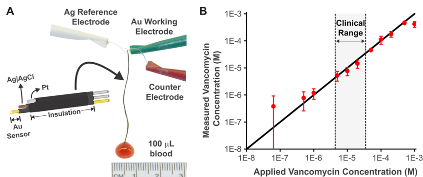
Figure 3. Using \sim 200\ \mu\text{m} -diameter, 3 mm-long (active sensing area) E-AB sensors, we have performed the calibration-free measurement of vancomycin in finger-prick-scale volumes ( 100\ \mu\text{L} ) of whole blood. (A) To achieve this, we employed sensors fabricated using 75\ \mu\text{m} -diameter gold, silver, and platinum wires that can easily be immersed in small volumes. (B) Using the nonresponsive 29 square-wave frequency (Figure 2B), we achieve clinically relevant ( \pm 20\% ) precision in the measurement of vancomycin over its entire clinical concentration range via a rapid (seconds) and single step. The asymmetry of the error bars is due to the use of a logarithmic y axis.
