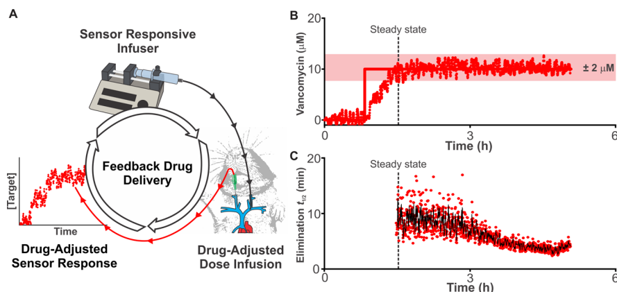
Figure 5. E-AB measurements support feedback-controlled drug delivery, supporting in turn high-precision control over plasma drug levels. (A) For this, we use seconds-resolved E-AB measurements as the input to a proportional–integral–derivative (PID) controller that computes the dosing rate required to best reach the desired plasma concentration administered via a PID-controlled drug-delivery infuser. (B) Using this approach, we can maintain a plasma vancomycin concentration within 2 \mu\text{M} of, as shown here, a 10 \mu\text{M} set point for more than 5 h, a duration that is limited by animal welfare concerns rather than by sensor performance. (C) We maintain this concentration in the face of \sim 3 -fold variation in the drug's elimination rate (calculated using the instantaneous infusion rate estimated by the PID); the black trace represents a 27 s (i.e., 3-point) rolling average.
