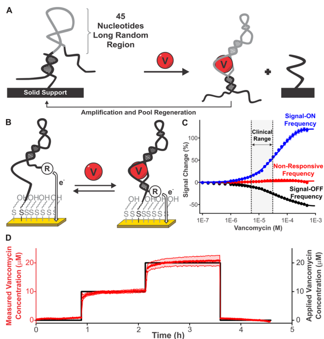
Figure 2. We demonstrate here the fabrication of a new, vancomycin-detecting E-AB sensor. (A) To achieve this, we first performed a solution-phase aptamer selection scheme that utilizes a key stem-loop closing step. Briefly, this starts with a single-stranded, surface-attached sequence partially complementary to a fixed region in a library pool of \sim 10^{14} distinct sequences flanked by two amplification regions and a random region of 45 nucleotides (in gray). Sequences that respond to the presence of target by detaching from their complement (presumably due to an intramolecular binding-induced conformational change) are then recovered, amplified, reconverted into a single-stranded library, and subjected to more rounds of selection. To measure the affinity of the resulting aptamer, we modified its sequence with a fluorophore and hybridized it using the partially complementary quencher-modified sequence (Figure S1). Titrating this with vancomycin further releases the complement sequence, thus increasing the measured fluorescence producing a dissociation constant ( K_D ) of \sim 0.1 \mu\text{M} . (B) We adapted the aptamer to the E-AB platform, which relies on a binding-induced change in the electron transfer kinetics of a redox reporter-modified (i.e., represented as “R”, which stands for methylene blue), surface-attached aptamer to produce a change in electron transfer rate that can be monitored using square-wave voltammetry. (C) Due to the dependence of electron transfer kinetics on the presence of target, the relative response of the vancomycin sensor is a strong function of square-wave frequency, producing “signal-off,” “signal-on,” or “nonresponsive” behaviors 28–30 that cover the clinically relevant range concentrations 36 in undiluted, flowing whole blood. (D) Using the output at the nonresponsive frequency and the constants \alpha (the ratio of the current at the nonresponsive frequency and at the responsive frequency at zero target concentration), K_D (the dissociation constant of the aptamer), and \gamma (signal gain) for vancomycin-detecting E-AB sensors (as a class), we can determine the concentration of vancomycin without the need for calibrating each individual device (see Table S1 for more details). 29 Doing so returns measured vancomycin concentrations within 20% of the applied concentration. The “error bars” shown here and those reported or illustrated elsewhere in this paper reflect 95% confidence intervals estimated from replicate measurements conducted on five independently fabricated sensors.
