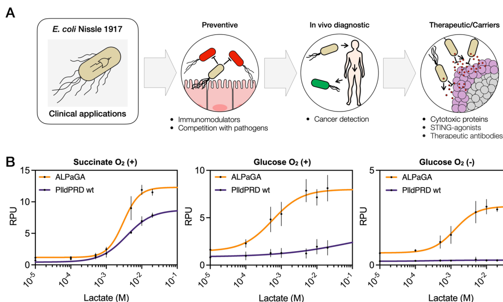
Figure 3. ALPaGA performance in the probiotic strain E. coli Nissle 1917. (A) Current summary of the probiotic Nissle 1917 for clinical application. (B) Dose–response functions of the PldPRD wt biosensor compared to the engineered ALPaGA sensors in different combinations of lactate, succinate, and glucose under aerobic (+O 2 ) or anoxic (–O 2 ) conditions. The fit of the curve was obtained from the mean of three different experiments performed in three different days. Error bars: +/– SD. RPU: reference promoter units. Response parameters are provided in Table 2.
