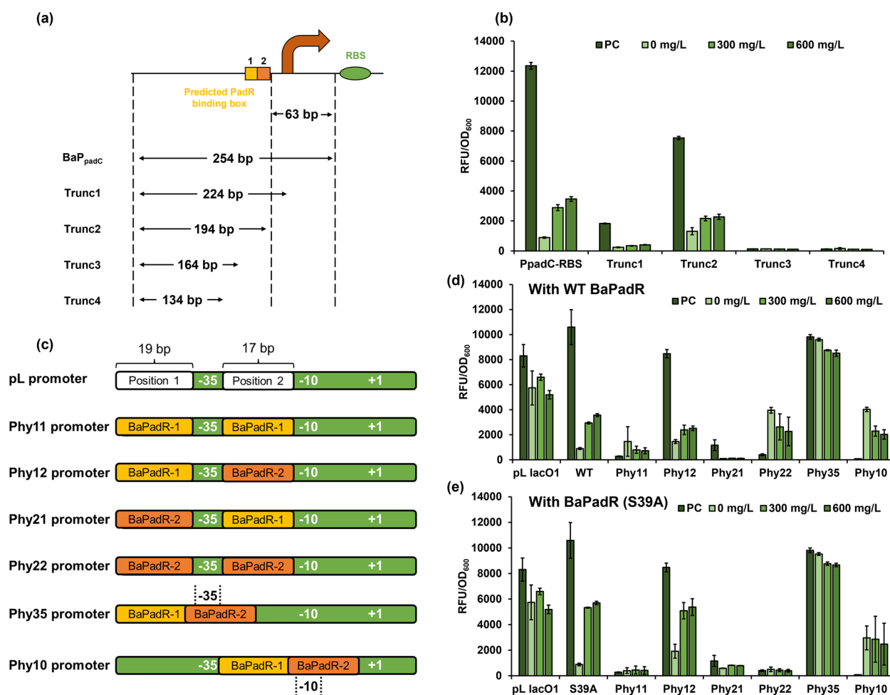
Figure 4. Identification of potential PadR binding box in the BaPpadC promoter and hybrid promoter construction. (a) Schematic illustrations for the truncation of BaP padC promoter. (b) Dynamic performance of the truncated promoters. (c) Schematic illustration of the hybrid promoter design strategy. (d) Dynamic performance of the hybrid promoters with WT BaPadR. (e) Dynamic performance of the hybrid promoters with BaPadR (S39A). All data represent the mean of 3 biologically independent samples and error bars show standard deviation.
