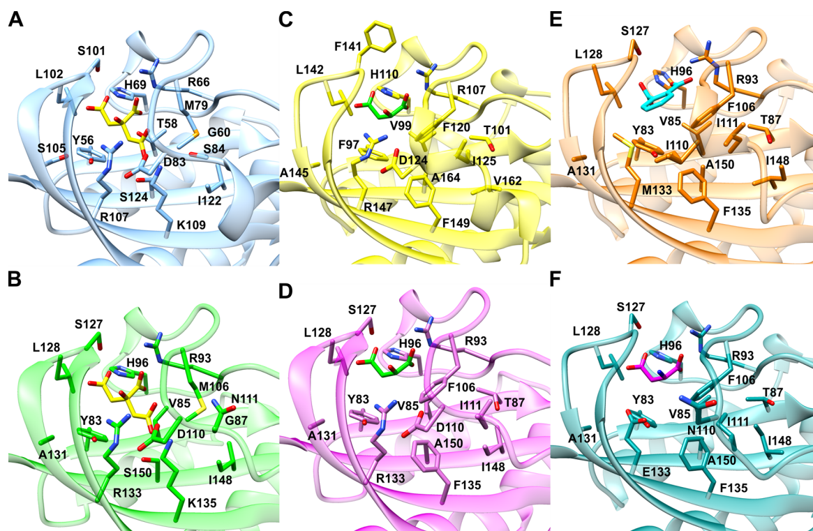
Figure 1. Structures and models of GtCitAP variants and homologues. (A) Crystal structure of the sensory CitA domain of K. pneumoniae 26 in ribbon presentation. Residues located in the binding site of the citrate ligand (yellow) are displayed as sticks. (B) Homology model of GtCitAP based on the crystal structure shown in (A). The position of the citrate ligand (yellow) was taken from the template structure. (C) Crystal structure of EcDcuSP . 41 The ligand L-malate is shown in green. (D) Homology model of GtMalAP based on the EcDcuSP structure shown in (C). The position of the ligand L-malate (green) was taken from the template structure. (E) Homology model of GtPhtAP based on the EcDcuSP structure shown in (C). The position of the ligand phthalate (cyan) was obtained by molecular docking with the ROSETTA server 52 and selected due to similar positioning of the carboxyl functions of phthalate compared to L-malate in the template structure. (F) Homology model of GtAspAP based on the EcDcuSP structure shown in (C). The ligand L-aspartate is shown in the same position as the isosteric ligand L-malate in the template structure.
