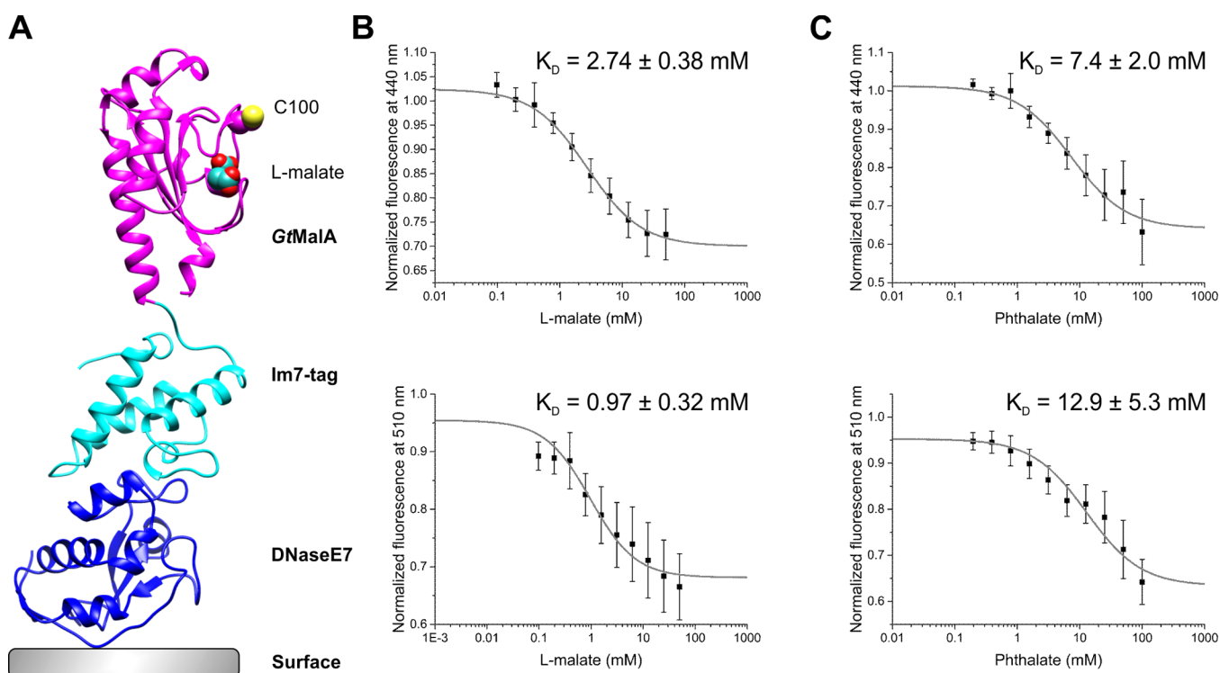
Figure 3. Characterization of GtCitAP variants immobilized on DNaseE7-coated surfaces. (A) Schematic structure of immobilized GtMalAP -D100C based on the homology model shown in Figure 1 and the crystal structure of the complex between DNaseE7 and Im7. 46 DNaseE7 (blue) was covalently coupled to the surface of maleic anhydride-activated microplates. GtMalAP -D100C (magenta) is attached to the surface via the high affinity interaction between its N-terminal Im7-tag (cyan) and the immobilized catalytically inactive DNaseE7-HS45A domain (residues 444–S76 of colicin E7). The ligand L-malate (red & cyan) and C100 (yellow), to which the label is attached, are shown as spheres. (B) The fluorescence of immobilized DACM-labeled GtMalAP -D100C at 440 nm (top) and the fluorescence of immobilized Dansyl-labeled GtMalAP -D100C at 510 nm (bottom) was fitted to a 1:1 Langmuir binding isotherm (gray curves) for determination of the affinity. The fluorescence of each well was normalized to its fluorescence in PBS and averaged for each concentration. Error bars represent standard deviations of at least four wells. Apparent K_D values are given with standard errors obtained from the fit. (C) Respective fits for DACM-labeled (top) and Dansyl-labeled (bottom) GtPhtAP -D100C and the ligand phthalate.
