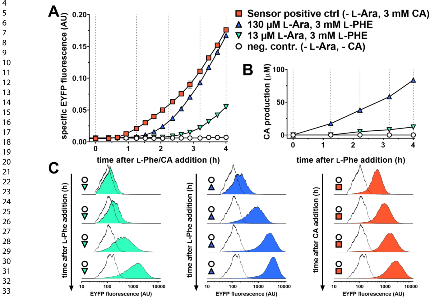
Figure 2. Influence of induction of heterologous xal TC expression with 13 \mu M L-Ara or 130 \mu M L-Ara on biosensor response and CA production in E. coli pSenCA pBAD- xal TC . After cultivation for 3 h in presence of different L-Ara concentrations, either 3 mM L-Phe (circles and triangles) or 3 mM CA (squares) was added. Samples were taken at four time points depicted by dotted lines (A) Specific fluorescence is shown (EYFP fluorescence \times biomass formation -1 , arbitrary units). (B) CA concentration in E. coli culture supernatants. (C) FACS measurement of EYFP fluorescence of 62,000 representative single cells in the histogram representation. Abbreviations: CA, trans -cinnamic acid; L-Ara, L-arabinose and L-Phe, L-phenylalanine.
