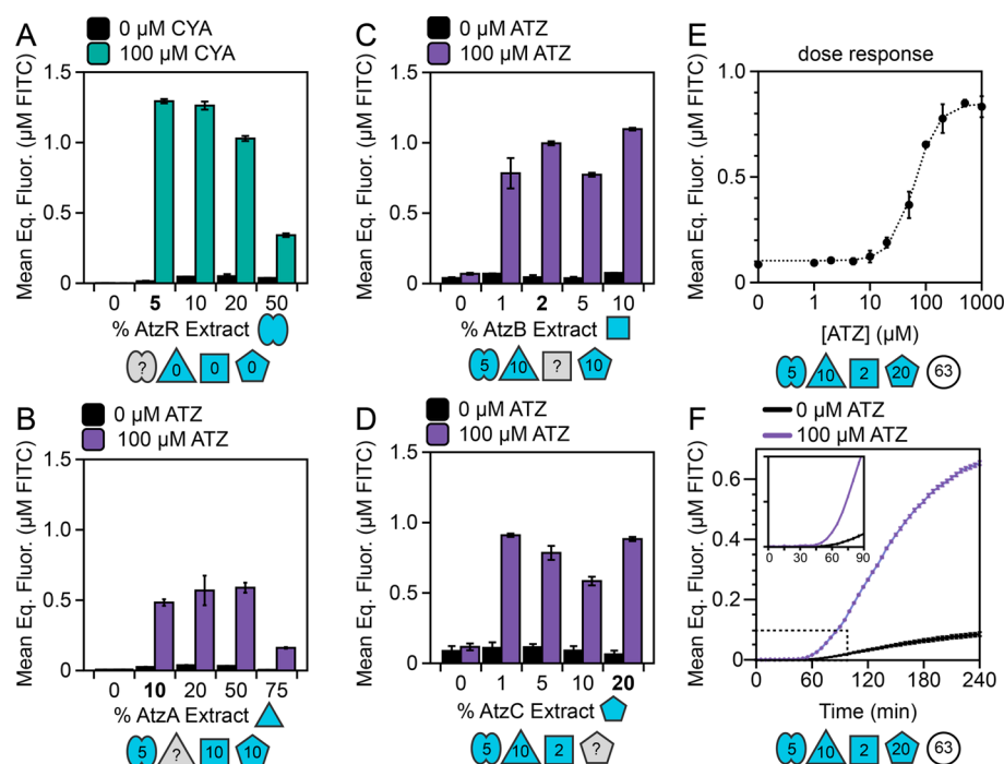
Figure 2. Optimization of the cell-free atrazine sensor. (A–D) Iterative optimization of the ratios of the AtzR, AtzA, AtzB, and AtzC extracts in the final sensor mixture reveals that the optimal fold induction is achieved at 5% AtzR-enriched, 10% AtzA-enriched, 2% AtzB-enriched, 20% AtzC-enriched, and 63% unenriched. Symbols below each plot denote the percentage of AtzR (bilobe), AtzA (triangle), AtzB (square), AtzC (pentagon), and blank (circle) extracts included in each experiment. Blank extract was added to make 100% in each condition. Each reaction contained 10 nM of the reporter DNA template from Figure 1. (E) Atrazine dose–response curve for the optimized sensor, measured by taking defined end point samples (4 h) from biosensor reactions containing the indicated amounts of atrazine, suggests that the overall limit of detection is around 20 \mu\text{M} , which is consistent with previous results reported for the cell-free cyanuric acid sensor. 12 The dashed line represents a sigmoidal fit to the data calculated by ordinary least-squares regression (refer to the Materials and Methods). (F) sfGFP fluorescence can distinguish the ON from OFF state within 1 h in the presence of 100 \mu\text{M} atrazine, and at end point achieves approximately 7-fold induction. Inset represents the time between 0 and 90 min and signal between 0 and 0.1 \mu\text{M} FITC. Error bars represent the standard deviation of sfGFP fluorescence measurements from three technical replicates, correlated to a known linear FITC standard.
