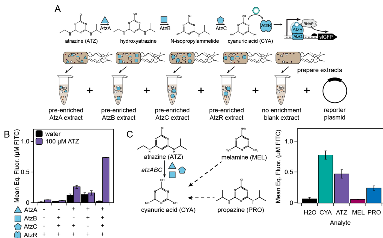
Figure 1. Design of a cell-free atrazine biosensor. (A) Atrazine is catabolized by a three-enzyme pathway into cyanuric acid, which can activate transcription through the AtzR transcription factor which recognizes an operator sequence within an engineered promoter. The four required proteins (three enzymes AtzA, AtzB, AtzC and the transcription factor AtzR) are separately overexpressed in strains of BL21 E. coli , then lysed and prepared into individual extracts, which can be mixed in fixed ratios to optimize detection of atrazine. (B) Cell-free detection of atrazine requires the presence of all three pathway enzymes. (C) The sensor is capable of detecting cyanuric acid and atrazine, as well as propazine, a triazine of similar chemical structure, but discriminates against melamine. CYA = cyanuric acid; ATZ = atrazine; MEL = melamine; PRO = propazine. All reactions include 10 nM of a fluorescent reporter DNA template and 100 \mu\text{M} of the respective triazine analytes. Error bars represent the standard deviation of sfGFP fluorescence measurements from three technical replicates, correlated to a known linear fluorescein isothiocyanate (FITC) standard.
