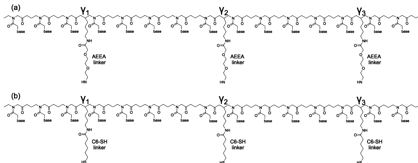
Figure 3. \gamma -PNA molecules with linker molecules attached at three \gamma -points ( \gamma_1 , \gamma_2 , and \gamma_3 ) on the AEG-backbone: (a) 2-aminoethoxy-2-ethoxy acetic acid (AEEA) with amine end group for attachment to \text{SiO}_2 surfaces; (b) hydrocarbon chain linker with thiol end group (C6-SH) for attachment to Au surfaces.
