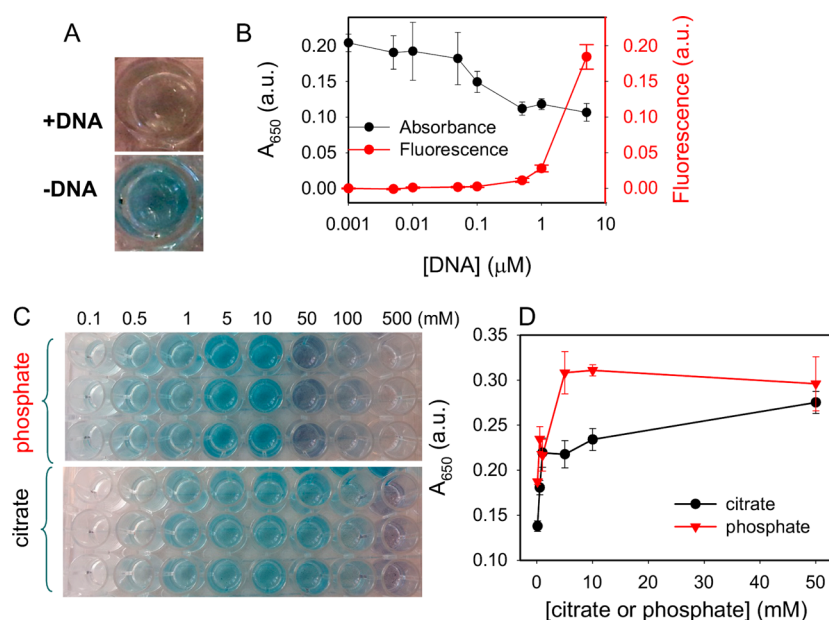
Figure 4. (A) Color of TMB sample mixed with nanoceria in the presence and absence of 5 \mu M DNA. (B) Quantification of color by UV-vis spectrophotometer and the change of DNA fluorescence in this mixture. The FAM-labeled DNA1 was dissolved in 10 mM acetate buffer, pH 4. The nanoceria concentration was 0.01% or 430 nM. (C) Color of TMB samples mixed with nanoceria in increasing concentrations of phosphate or citrate buffers (pH 4). Deep blue colors at high buffer concentrations are due to precipitation. (D) Quantification of oxidation of the samples in C by monitoring absorbance at 650 nm.
