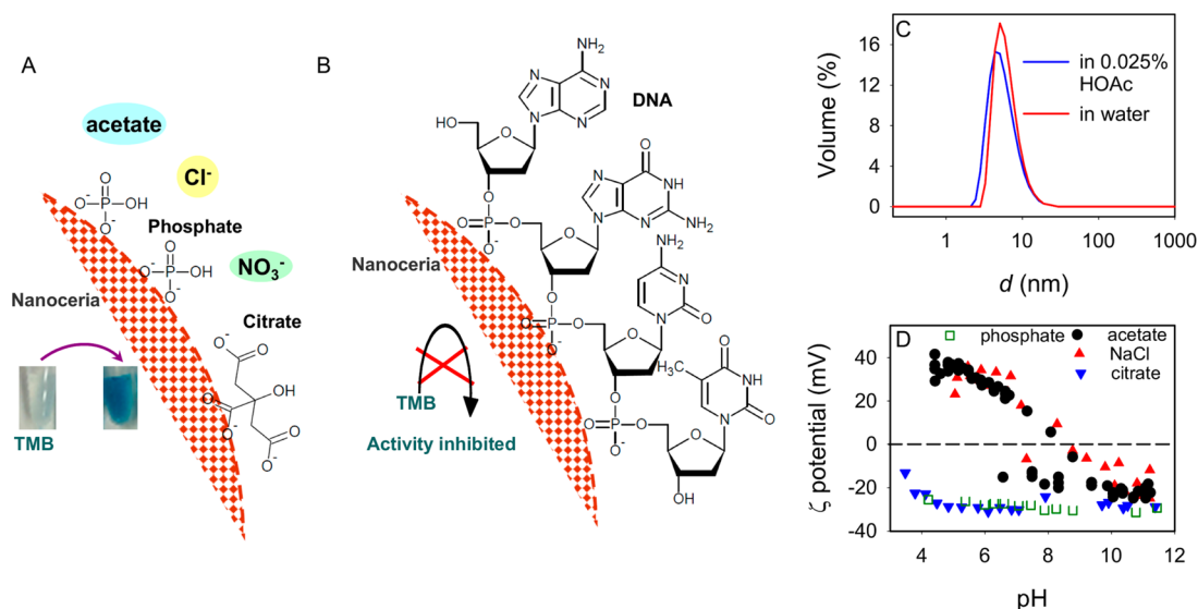
Figure 1. (A) Cartoon showing that nanoceria can tightly adsorb phosphate and citrate, resulting in negatively charged surface, but with low affinity with acetate, chloride, and nitrate. Its oxidase activity is retained in all these buffers to convert TMB into a blue product. (B) Nanoceria adsorbs DNA via the phosphate backbone. The oxidase activity is inhibited upon DNA adsorption. (C) DLS spectra of nanoceria dispersed in an acidic buffer or in water. (D) \zeta -potential of nanoceria as a function of pH in various buffer conditions (10 mM phosphate, citrate, or acetate). The sample marked with NaCl (10 mM) does not contain any buffer.
