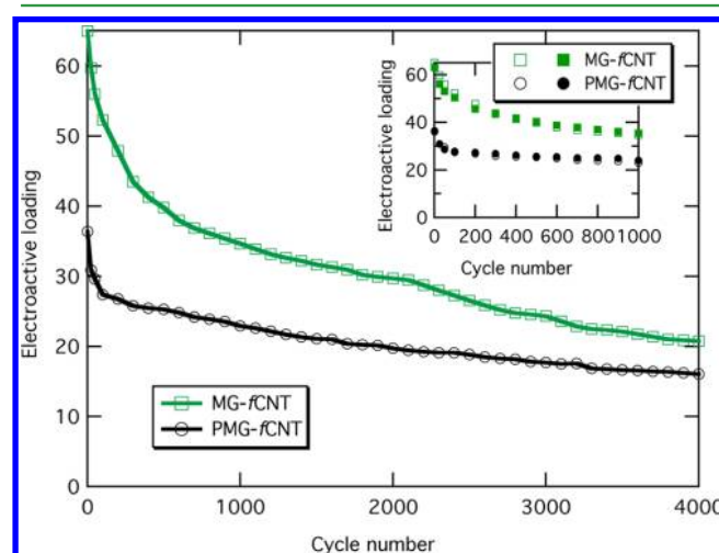
Figure 9. Stability of modified electrodes as measured by cyclic voltammetry (CV) at 900 rpm, 0.1 M phosphate buffer pH 7.45, 30 °C. Electroactive loading was obtained by integration of CV redox peaks, assuming a two-electron redox reaction.
