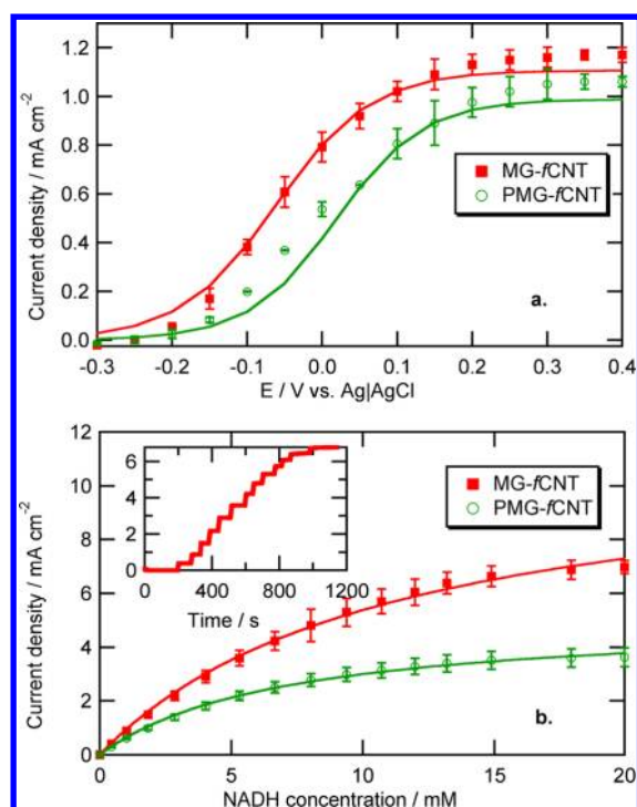
Figure 6. NADH electrocatalysis activity of MG-fCNT and PMG-fCNT at 900 rpm in 0.1 M phosphate buffer pH 7.45, 30 °C. (a) Polarization curve in 1 mM NADH; (b) NADH concentration study at 50 mV vs Ag/AgCl. Inset: time-dependent curve on MG-fCNT.
