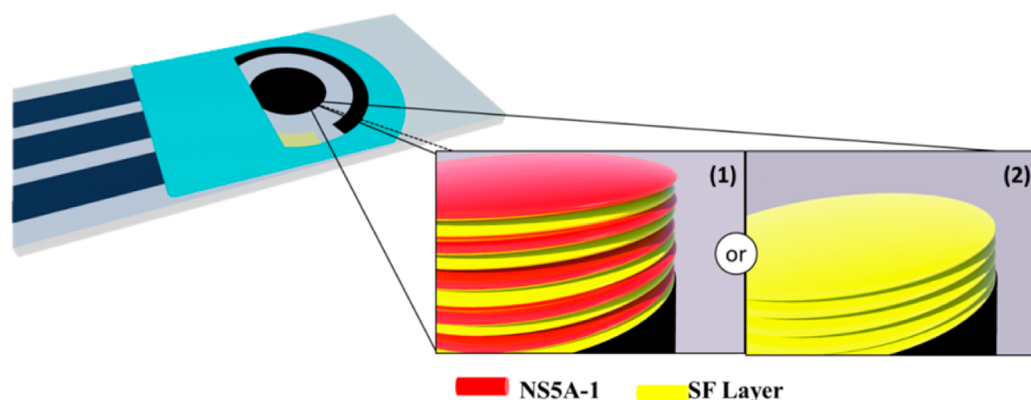
Figure 6. Schematic representation of five-layer LbL film of SF/NS5A-1 (1) and RSF (2) assembled onto carbon screen-printed electrodes. Reproduced with permission from ref 176.
