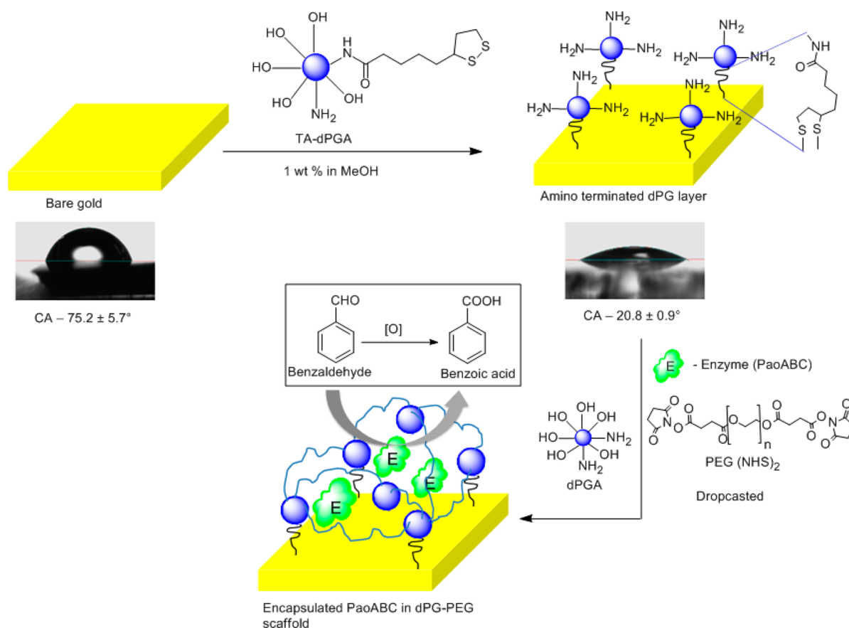
Figure 1. Scheme displaying the modification steps involved in the construction of a dPG-PEG scaffold ( n = 34, 136 , and 227 ; PaoABC electrochemical biosensor) on gold surfaces. Inserted pictures: static water contact angles of the bare and TA-dPGA-modified gold surfaces.
