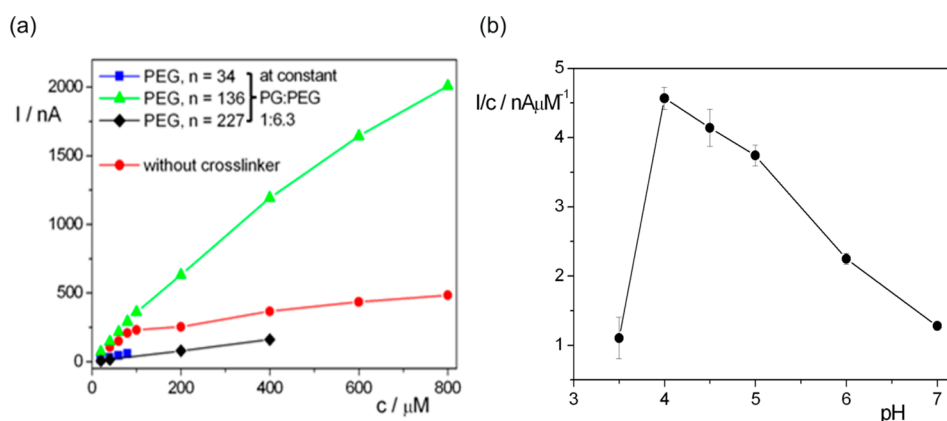
Figure 2. (a) Effect of the length of the cross-linker used for PaoABC biosensor preparation on the amperometric signal of BA with a concentration range of 20–800 \mu M. (b) Effect of the pH on the sensitivity of the amperometric BA measurement at the PaoABC biosensor. Measurements were performed in a citrate phosphate buffer with pH 4.5 in the presence of 2 mM mediator HCF at a potential of +250 mV vs Ag/AgCl.
