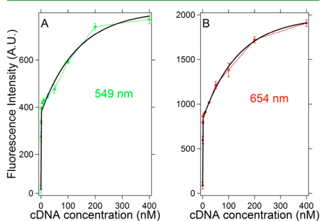
Figure 7. Representation of the maximum fluorescence intensity bands measured at 549 nm (A) and 654 nm (B) of the UCNPs@SiO 2 -ssDNA nanoparticles as a function of the complementary ssDNA concentration.
