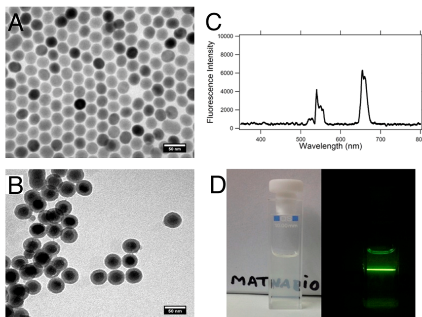
Figure 1. (A) TEM micrograph of monodisperse \text{NaYF}_4:\text{Yb,Er} nanoparticles. (B) TEM micrograph of monodisperse and individually coated \text{NaYF}_4:\text{Yb,Er}/\text{SiO}_2 nanoparticles. Scale bars are 50 nm. (C) Fluorescence spectrum of a diluted solution in ethanol of the silanized upconversion nanoparticles when excited with a continuous wave 980 nm laser. (D) Pictures taken of the diluted solution of silanized upconversion nanoparticles in ethanol without laser excitation (left) and the same solution under the excitation of a cw 980 nm laser (right). The room light was turned off to take this picture.
